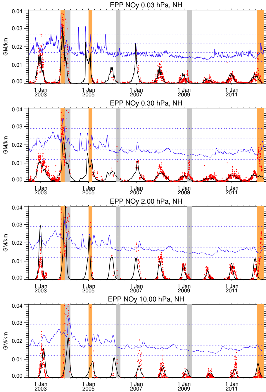
Figure 3a. Observed (red diamonds) and fitted (black solid) temporal evolution of hemispheric EPP-NO y amounts during 2002–2012 at the pressure levels 0.03, 0.3, 2, and 10 hPa (top to bottom) in the NH. \overline{A_p}(z, t) of the empirical model for quiescent dynamical conditions is shown with blue lines (dotted blue lines indicate A_p levels with spacing of 5 A_p units). Shaded areas have been excluded from the fit due to perturbed dynamics (i.e., SSW and ES events, grey) and large SPE events (orange). Note that the y-axis range does not cover the very high NO y amounts encountered in the NH 2003/04 winter.
