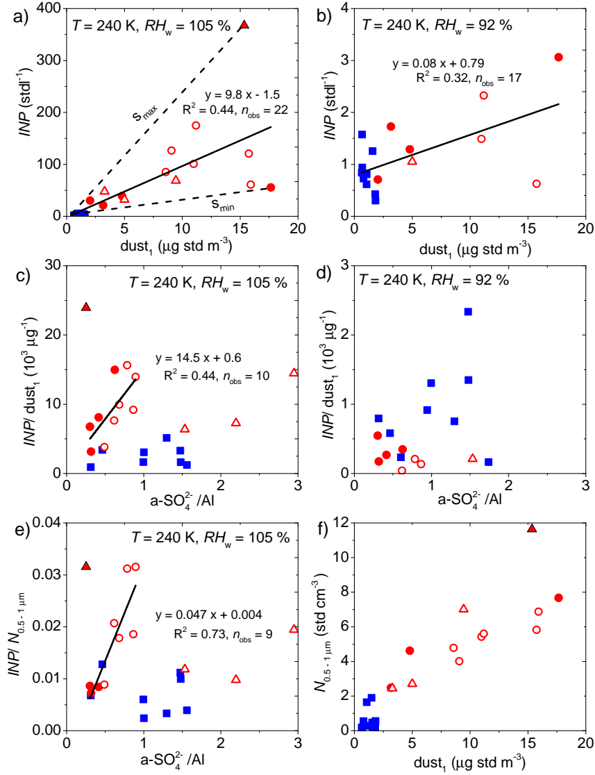
Figure 10. a) and b): correlation of [INP] with dust 1 ; c) and d): correlation of [INP]/\text{dust}_1 with \text{a-SO}_4^{2-}/\text{Al} ; e) correlation of [INP]/N_{0.5-1\mu\text{m}} with \text{a-SO}_4^{2-}/\text{Al} ; f) N_{0.5-1\mu\text{m}} versus dust 1 . Plots a), c) and e) show condensation mode [INP] and b) and d) deposition mode [INP] at 240 K. All samples were taken between 22:00-06:00 UTC. Blue squares indicate Atlantic air masses, red circles Sahara influence (open: 2013, filled: 2014) and triangles denote outliers (see text for details).
