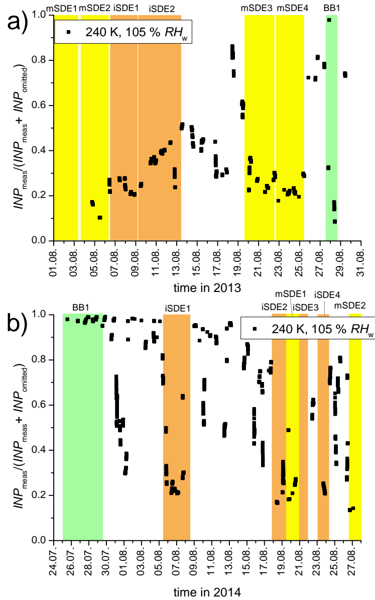
Figure 12. a) Time series in 2013 and b) in 2014 of the ratio of measured [INP] to total potential [INP] , i.e. the sum of measured [INP] and the calculated omitted [INP] due to the use of the impactor. Color coding refers to events described in Fig. 3 and Fig. 4.
