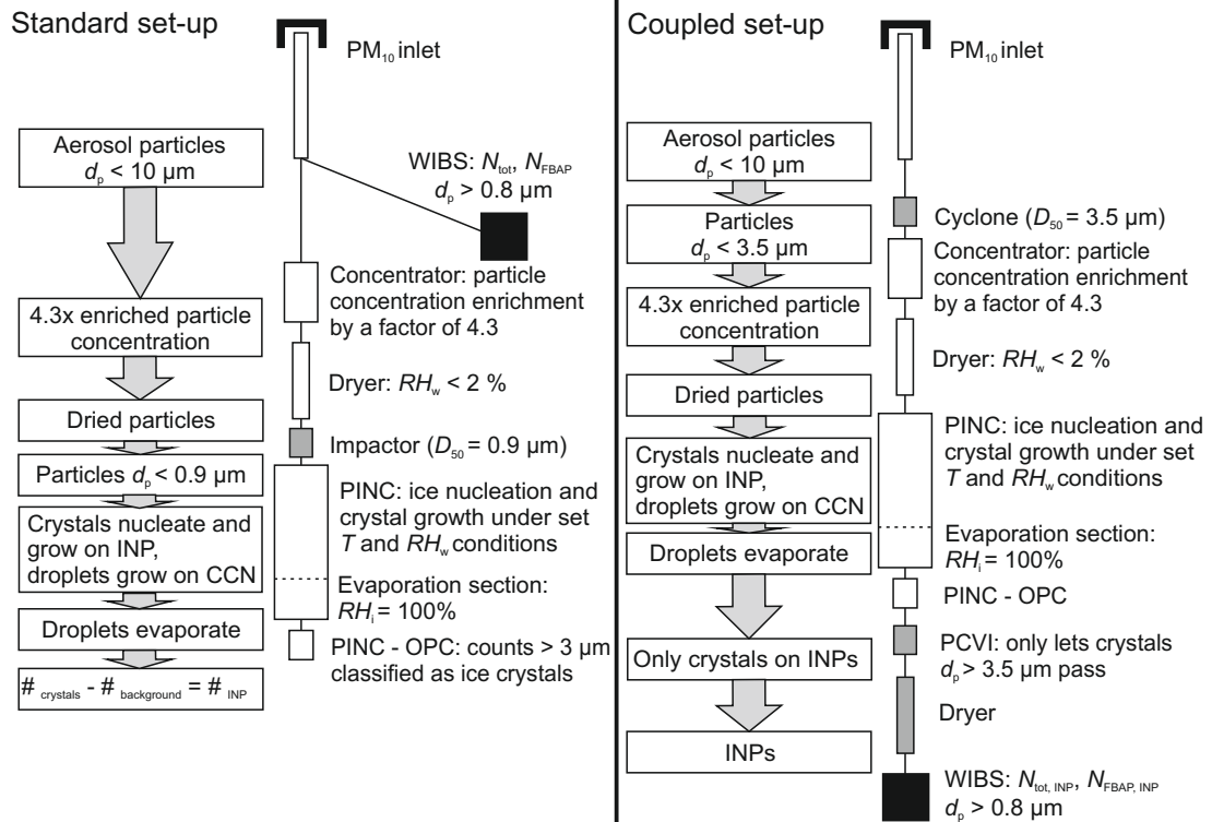
Figure 1. Left panel: standard set-up of PINC and WIBS during CLACE2014. Right panel: set-up for PINC-PCVI-WIBS coupling. Note the different position of the WIBS (black box). The gray parts are changed between the two different set-ups. Adapted from Boose et al. (2016). See text for details.
