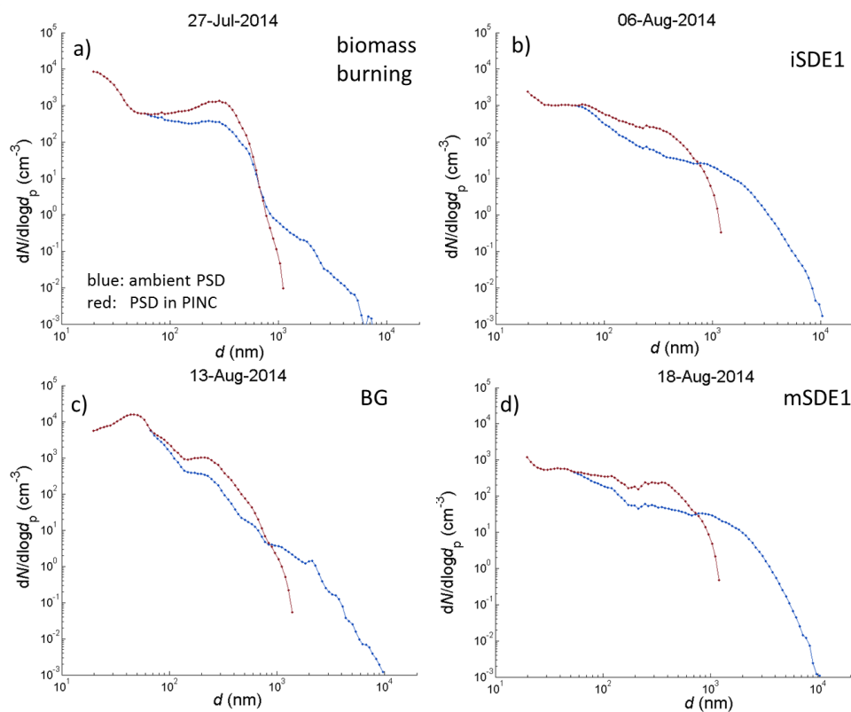
Figure 11. Effect of concentrator and impactor on aerosol particle size distribution (PSD) for different event types during CALIMA2014: a) biomass burning event b) intermediate Saharan dust event 1, c) background conditions and d) major dust event 1. In blue are the ambient PSDs, in red the corrected PSDs how they are inside of PINC. Each ambient PSD curve was measured at noon of the respective day.
