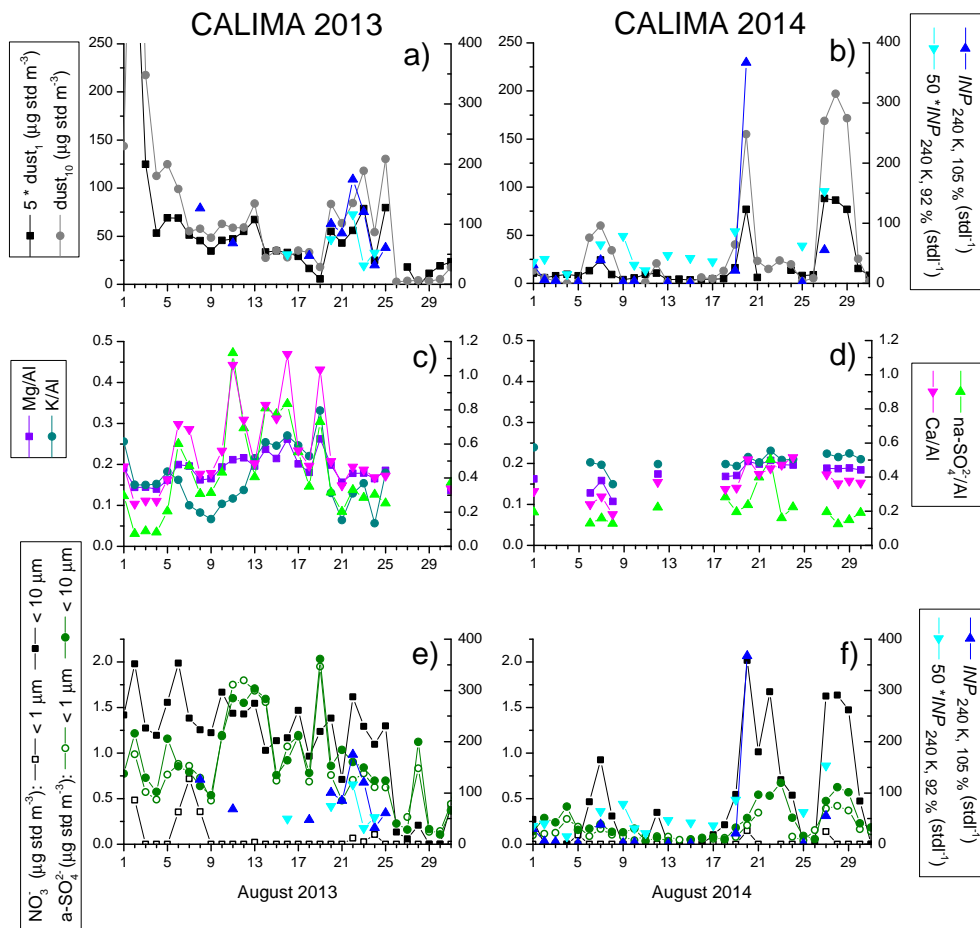
Figure 9. Time series of nighttime measurements during CALIMA2013 and CALIMA2014. y-axes labels indicate axes of the respective data in each row.
