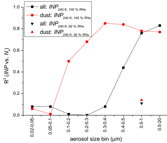
Figure 5. Correlation of [INP_{240\text{K}, 105\% RH_w}] and aerosol concentration ( N_x ) of particles of different sizes during CALIMA2014 for dust periods and all periods together. Also shown is the R^2 for [INP_{240\text{K}, 92\% RH_w}] with N_{0.5-1\ \mu\text{m}} .
