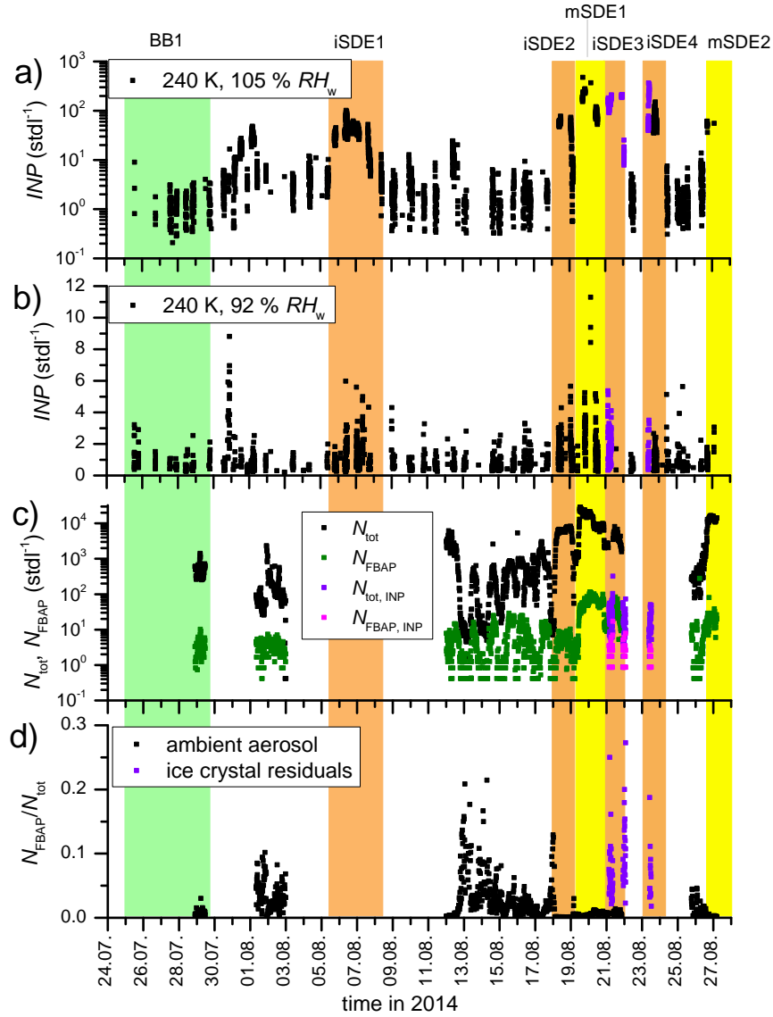
Figure 7. [INP] during CALIMA2014 in a) condensation and b) deposition mode at 240 K. Purple data points indicate times when the WIBS was connected downstream of PINC. c) Total and fluorescent particle concentration as measured by the WIBS in parallel (black and green) and in series with PINC (purple and magenta) d) Fluorescent to total particle concentration in parallel (black) and in series (purple) to PINC.
