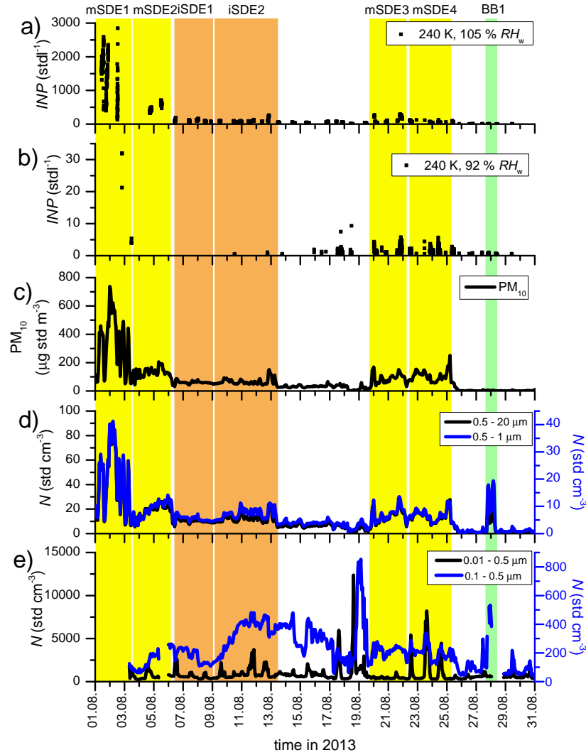
Figure 3. CALIMA2013: [INP] in a) condensation and b) deposition mode at 240 K. c) PM_{10} , d) aerosol particle number concentration as measured by the APS and e) as measured by the SMPS. Yellow shading indicates major dust events (mSDE, PM_{10} \geq 100 \mu\text{g std m}^{-3} ) and orange shading intermediate dust events (iSDE, 50 \leq PM_{10} \leq 100 \mu\text{g std m}^{-3} ). Minor dust events ( 20 \leq PM_{10} \leq 50 \mu\text{g std m}^{-3} ) are not indicated. Green shading indicates a biomass burning event (BB1).
