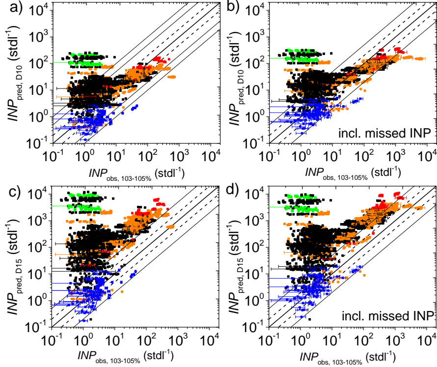
Figure 13. Observed [INP] from CALIMA2013 and CALIMA2014 at 105 % RH_w and from CLACE2014 at 103 % vs. predicted [INP] based on the parameterizations from a) and b) DeMott et al. (2010) and c) and d) DeMott et al. (2015). Green data points refer to biomass burning events, orange and red points to intermediate and major dust events, respectively, and black data points to the remaining time periods. CLACE2014 data are shown in blue. The 1:1 line is given as thick solid line, the dashed lines indicate a factor 2 and the thin solid line a factor of 5. The 95 % confidence interval given by DeMott et al. (2015) is about a factor of 4. For the predicted [INP] in a) and c) aerosol particle concentrations corrected for impactor and concentrator were used. For b) and d), the omitted potential INPs were included in the observed [INP] and ambient N_{0.5-20\mu m} were used for the predicted [INP] . Error bars are drawn for 100 random data points per plot. They include the uncertainties of the [INP] , n_s and aerosol size distribution measurements.
