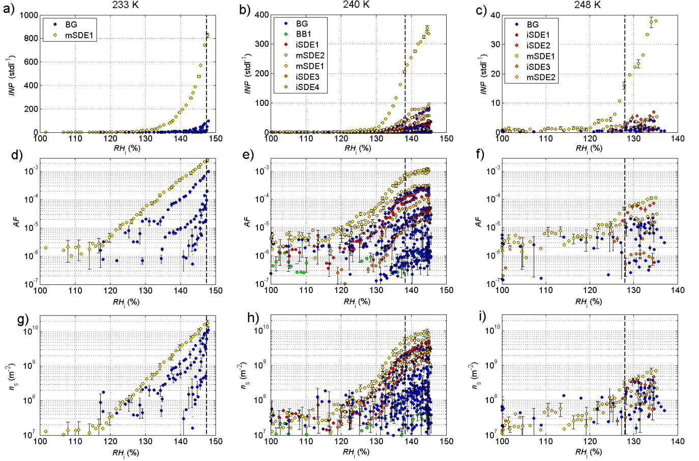
Figure 6. RH_i scans of [INP] , AF and n_s at 233 K, 240 K and 248 K during CALIMA2014. The dashed vertical lines indicate water saturation. Event types are the same as in Fig. 4 with the addition of BG for background conditions, i.e. not affected by Sahara dust or biomass burning. Error bars are drawn for every third data point.
