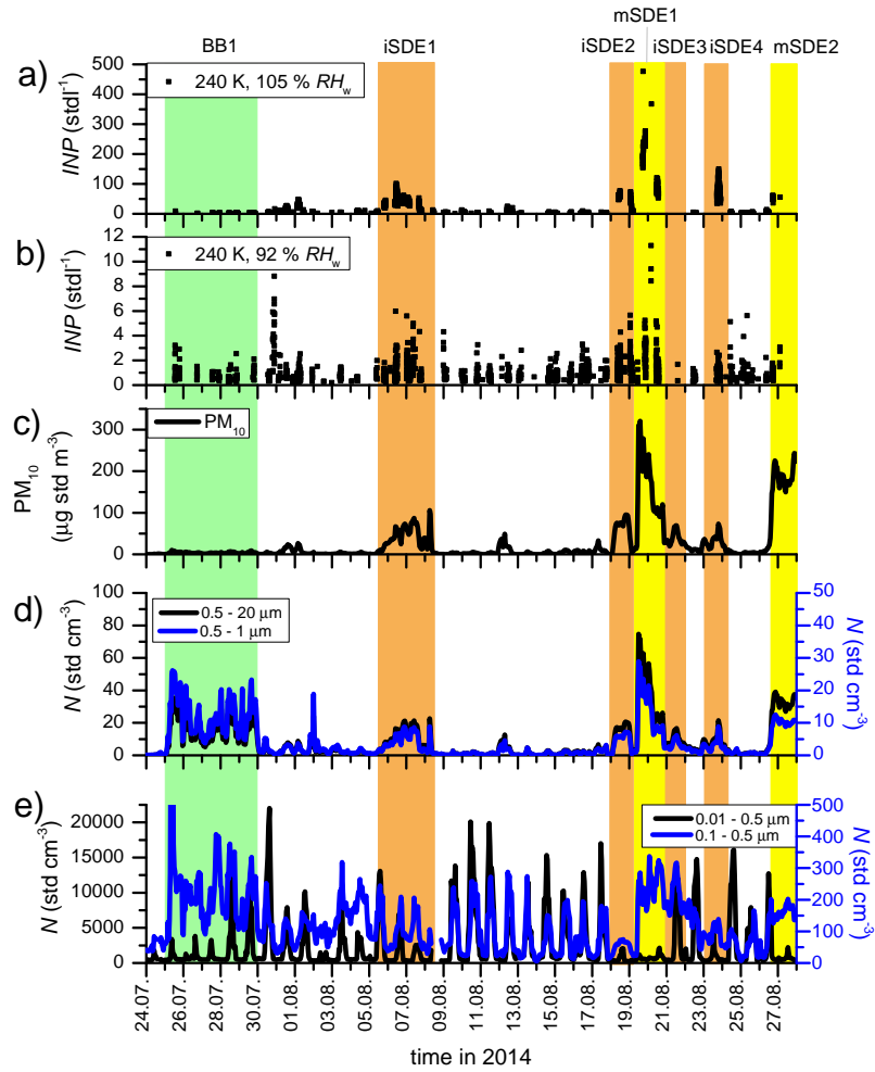
Figure 4. As in Fig. 3, but for CALIMA2014.
