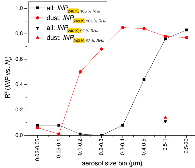
Figure 5. Correlation of [INP_{240K, 105\% RH_w}] and aerosol concentration ( N_x ) of particles of different sizes during CALIMA2014 for dust periods and all periods together. Also shown is the R^2 for [INP_{240K, 92\% RH_w}] with N_{0.5-1 \mu m} .
