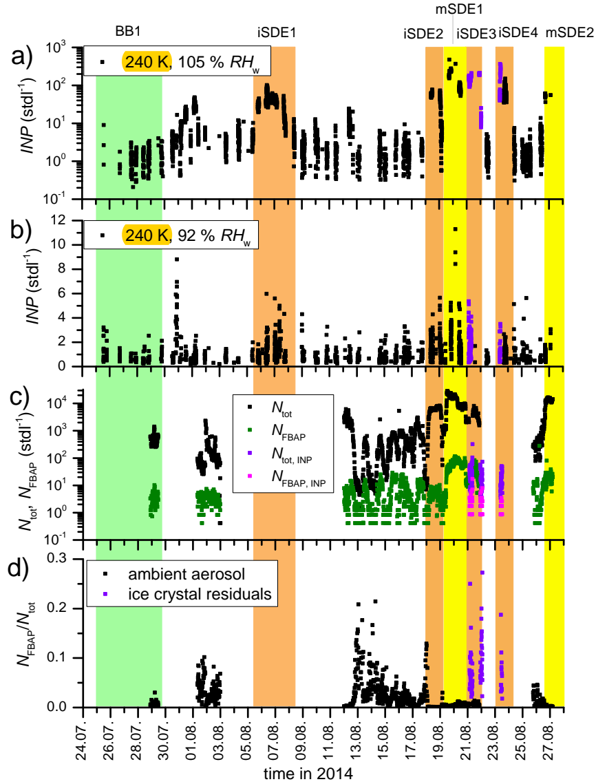
Figure 7. [INP] during CALIMA2014 in a) condensation and b) deposition mode at 240\text{ K} . Purple data points indicate times when the WIBS was connected downstream of PINC. c) Total and fluorescent particle concentration as measured by the WIBS in parallel (black and green) and in series with PINC (purple and magenta) d) Fluorescent to total particle concentration in parallel (black) and in series (purple) to PINC.
