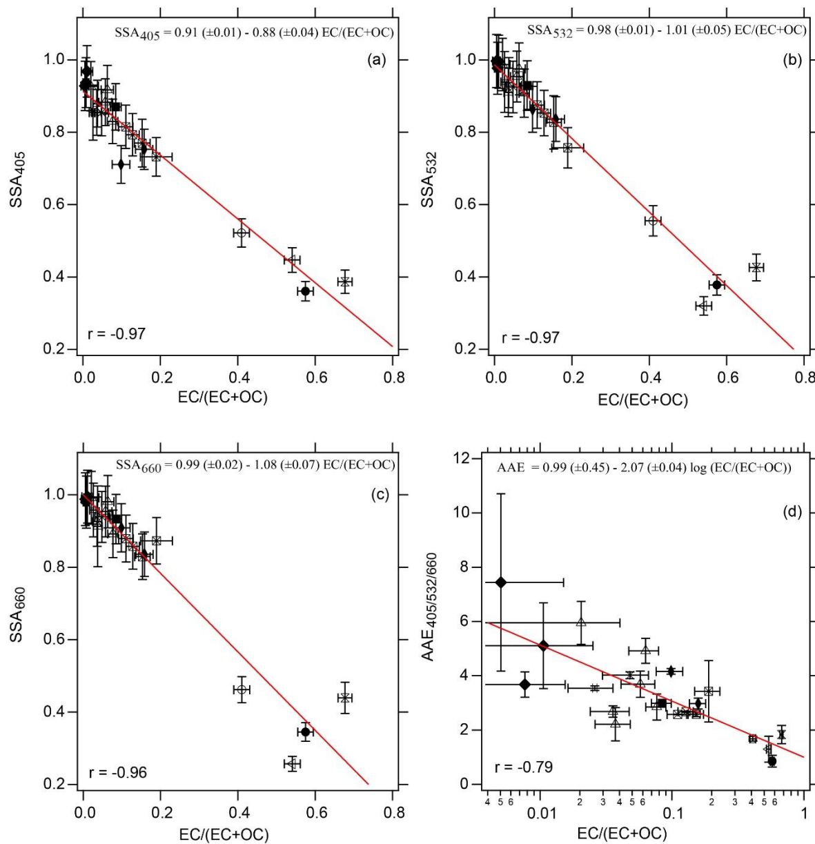
Figure 4. Same as Fig. 3 but for SSA plotted vs. \frac{EC}{(EC+OC)} . Equations for the fits are given in each panel.
