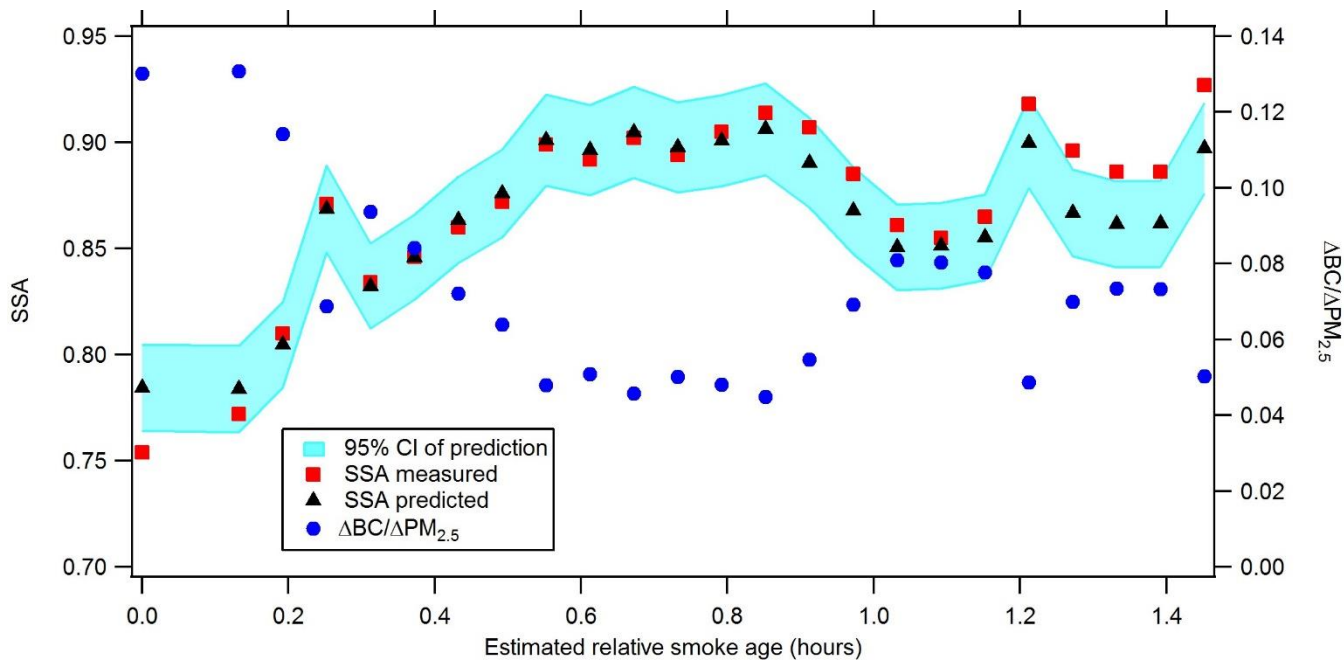
Figure 5. Measured (Yokelson et al., 2009) and predicted SSA at 532 nm for biomass burning emissions during the initial 1.4 hours of aging. Shaded region indicate the 95 % confidence interval of the predicted SSA.
