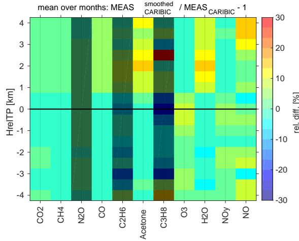
Figure 5. Mean relative differences of \text{MEAS}_{\text{CARBIC}}^{\text{smoothed}} and \text{MEAS}_{\text{CARBIC}} . \text{MEAS}_{\text{CARBIC}}^{\text{smoothed}} has been smoothed by interpolating between the 20 min mean values, the exact method being presented in App. ???. The relative differences correspond to the error in the climatologies of \text{MOD}_{\text{CARBIC}}^{\text{sampled}} due to the coarse model resolution. \text{N}_2\text{O} , \text{C}_2\text{H}_6 and \text{C}_3\text{H}_8 are measured by air samples with a low measurement frequency and therefore not considered here.
