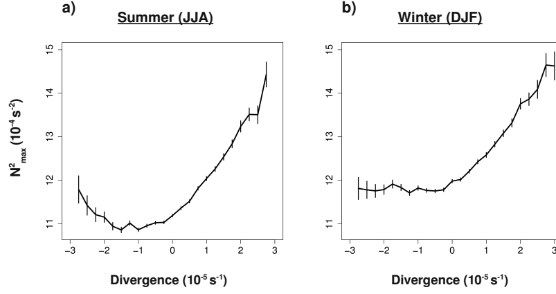
Figure 3. Diagrams of horizontal wind divergence versus TIL strength ( N_{max}^2 ) for the latitude band 10^\circ\text{S} - 10^\circ\text{N} . a) belongs to the summer season (JJA), and b) to the winter season (DJF). Vertical bars denote one standard deviation of the mean value.
