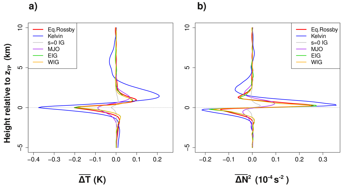
Figure 6. Winter (DJF) average signature of the different wave types, as the mean anomaly of (a) temperature and (b) N^2 in the equatorial zonal-mean vertical profiles ( 10^\circ\text{S} - 10^\circ\text{N} ).
