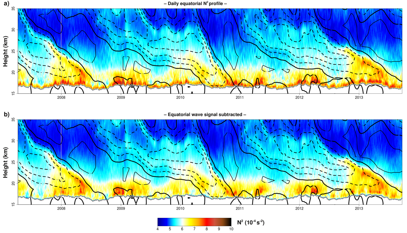
Figure 7. a) Daily evolution of the tropopause-based, equatorial ( 10^{\circ}\text{S} - 10^{\circ}\text{N} ) zonal mean N^2 vertical profile between 2007-2013 (colors) from COSMIC GPS-RO profiles. The grey line denotes the tropopause height ( TP_z ). Thin black contours denote positive (westerly) mean zonal wind, with a thicker contour for the zero line, dashed contours for negative (easterly) winds, and a 10m/s separation. To improve visibility, the winds are displayed with a running mean of \pm 15 days. No running mean is applied to the N^2 vertical profile or TP_z in order to allow the subtraction of the equatorial wave signal. b) Equatorial wave signal subtracted from the N^2 vertical profile.
