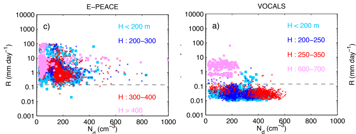
Figure 2: Scatter diagrams of cloud droplet number concentrations N_d and precipitation, R , for E-PEACE (left) and VOCLAS-TO Flights (right). Colors indicate cloud thickness H . The dashed line indicates an R value of 0.14 \text{ mm day}^{-1} .
