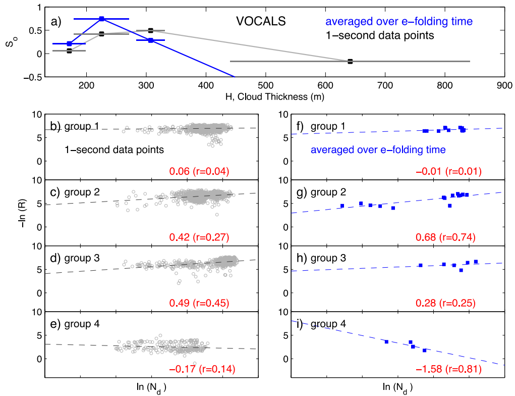
Figure 6. S_0 for VOCALS TO flight is calculated with 1-second data (grey) and cloud data that are averaged over an e-folding time for each H interval. The \ln(N_d) and -\ln(R) diagram is shown for each H interval. The horizontal bar in (a) indicates \pm 1\sigma . S_0 is calculated for the cloud data in groups with similar H (shown in Table 1).
