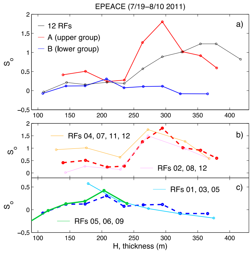
Figure 8. S_0 as a function of cloud thickness for (a) 12 E-PEACE flights, for groups A and B shown in Fig. 7. (b) S_0 , calculated with randomly resampled RFs within groups (b) A and (b) B. RFs indicate Research Flights.
