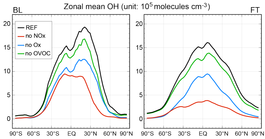
Figure 11: Zonal, annual mean OH concentrations calculated in the reference simulation (black) and by successively 5 excluding OH recycling through the \text{NO}_x , \text{O}_x and OVOC mechanisms.
