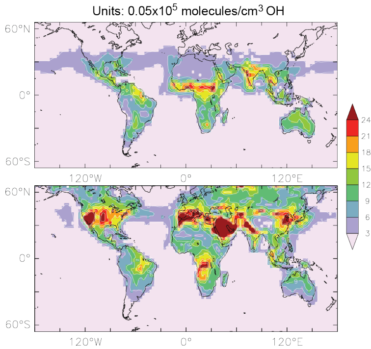
Figure 2: Nighttime OH in the boundary layer in January (top) and July (bottom). Color coding is the same as Fig. 1, but concentrations are scaled by a factor 20 ( \times 0.05 \cdot 10^5 molecules/cm 3 ).
