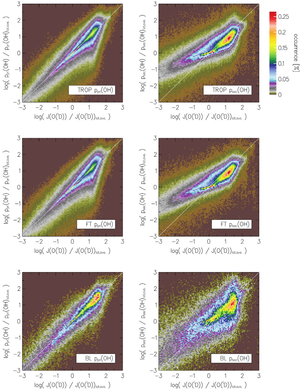
Figure 8: Correlation diagrams, showing P and S on the Y-axes as a function of the photo-dissociation rate of O_3 by OH , J(O^1D) , on the X-axes. Please notice the log/log scale. P is shown in the left panels and S in the right panels, in the 5 troposphere (top), FT (middle) and BL (bottom).
