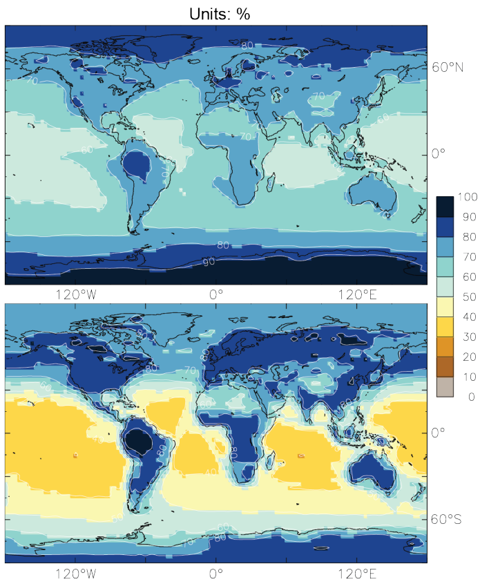
5 Figure 9: Annual mean OH recycling probability ( r in %) in the troposphere (top) and the BL (bottom).
