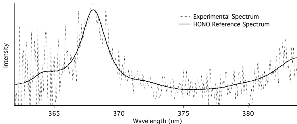
Figure 1: Experimental absorption spectrum fit with a reference HONO spectrum (Stutz et al., 2000) using DOASIS (Lehmann, 2009). This spectrum was measured at RH = 37% and represents a concentration of 2.17 \times 10^{11} molecules \text{cm}^{-3}
