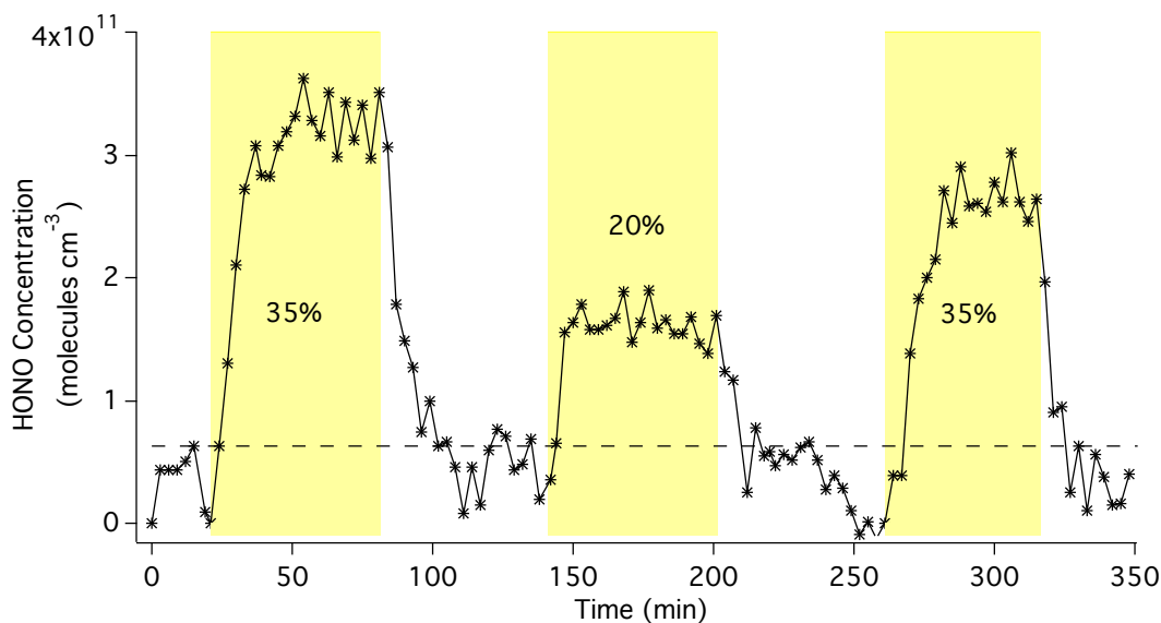
Figure 2: Time trace of an experiment where the sections highlighted in yellow indicate when the sample is exposed to light. The relative humidity in the chamber during each illumination period is indicated. The HONO detection limit is indicated by the dashed line.
