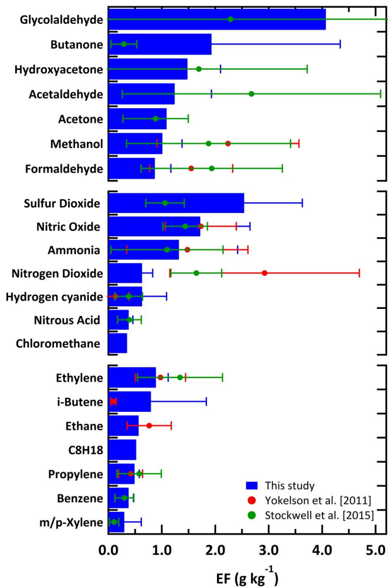
Figure 4. The emission factors (g/kg) and \pm one standard deviation for the most abundant OVOCs, NMHCs, and S-/N-containing compounds emitted from crop residue burns. The crop residue fires from other studies (Yokelson et al., 2011; Stockwell et al., 2015) are shown in red and green.
