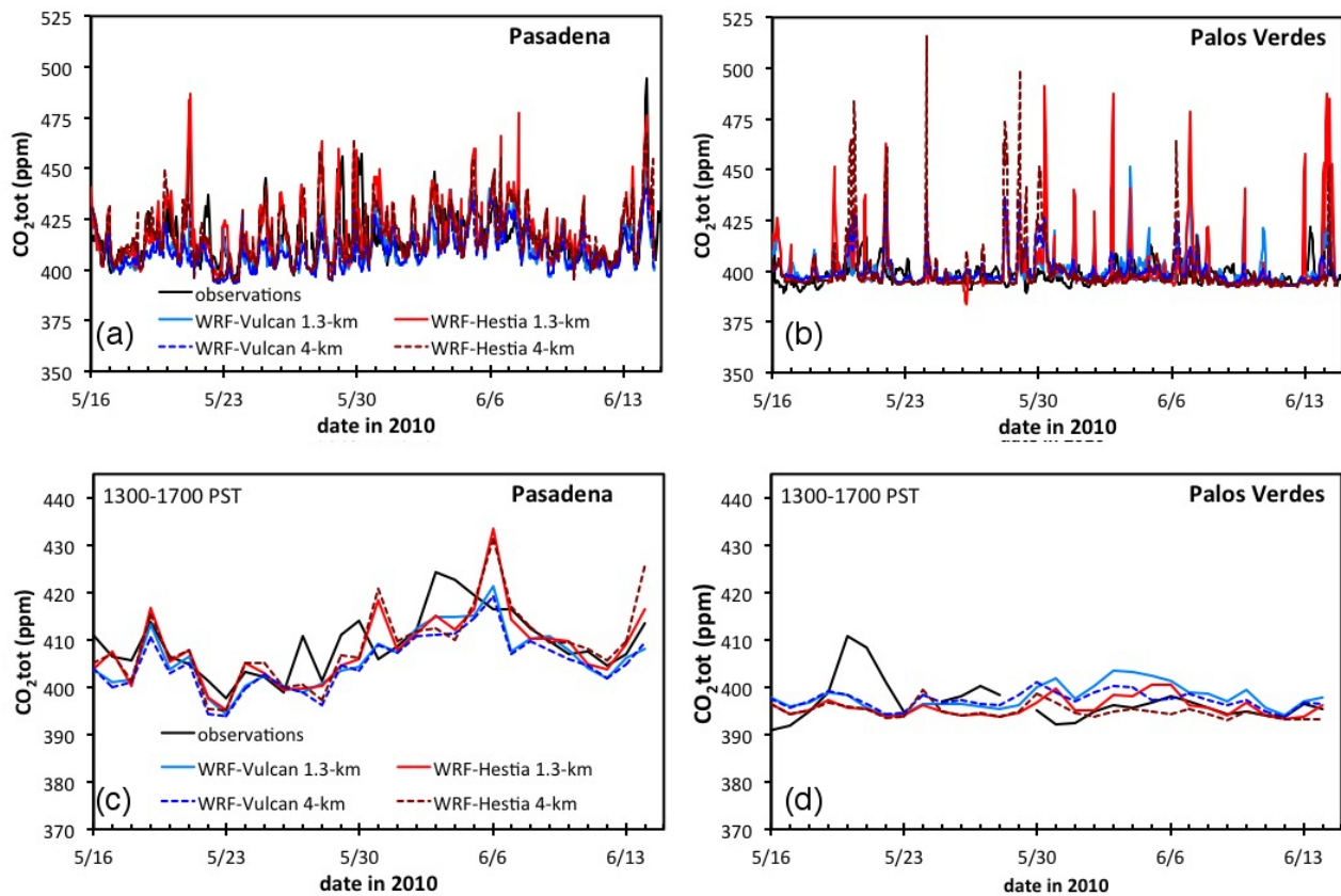
Figure 8. Comparison of the observed and modelled CO 2 concentrations at the (a and c) Pasadena and (b and d) Palos Verdes sites: (a and b) hourly time series, (c and d) daily afternoon averages for 1300-1700 PST.
