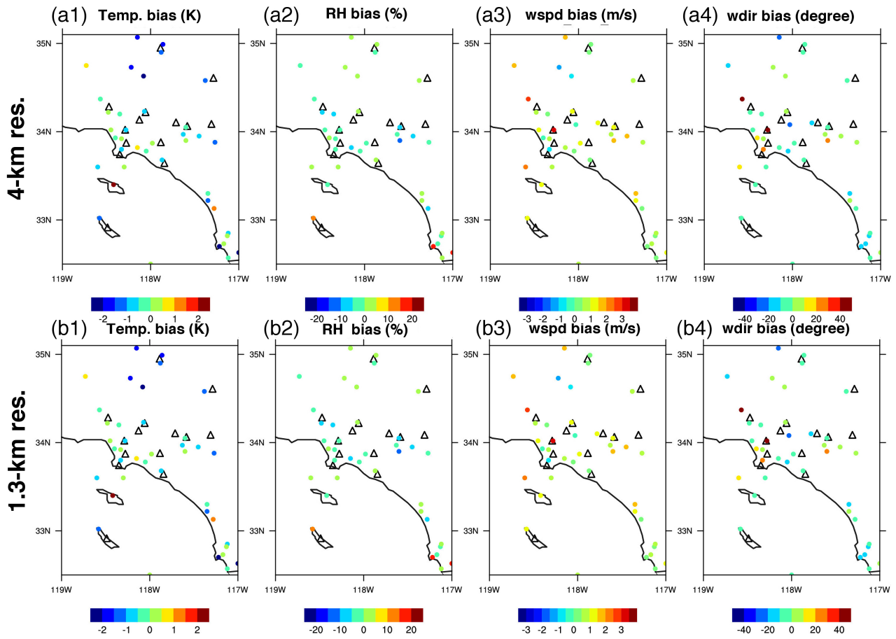
Figure 6. Bias maps of atmospheric state variables from the MYNN_UCM runs versus National Weather Stations (NWS) over the LA megacity (Model - NWS): (a1-a4) 4-km run; (b1-b4) 1.3-km run. Black triangles indicate the locations of the GHG measurement sites. Note daytime 1100-1700 PST only.
