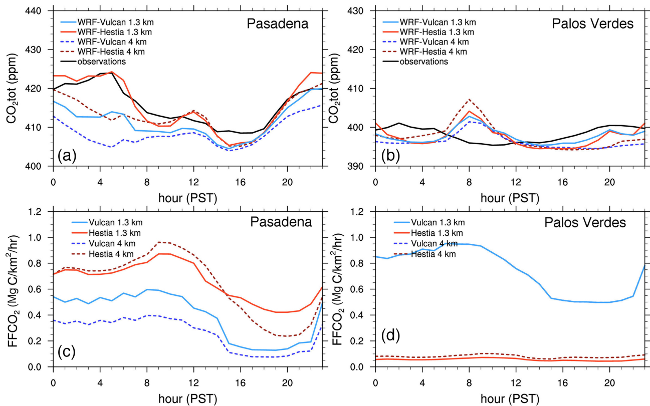
Figure 9. Averaged diurnal variation of observed and modelled \text{CO}_2 concentration and \text{FFCO}_2 emissions for the (a and c) Pasadena and (b and d) Palos Verdes sites during CalNex-LA. Note that Vulcan 4-km overlaps with Vulcan 1.3-km in Figure 9d.
