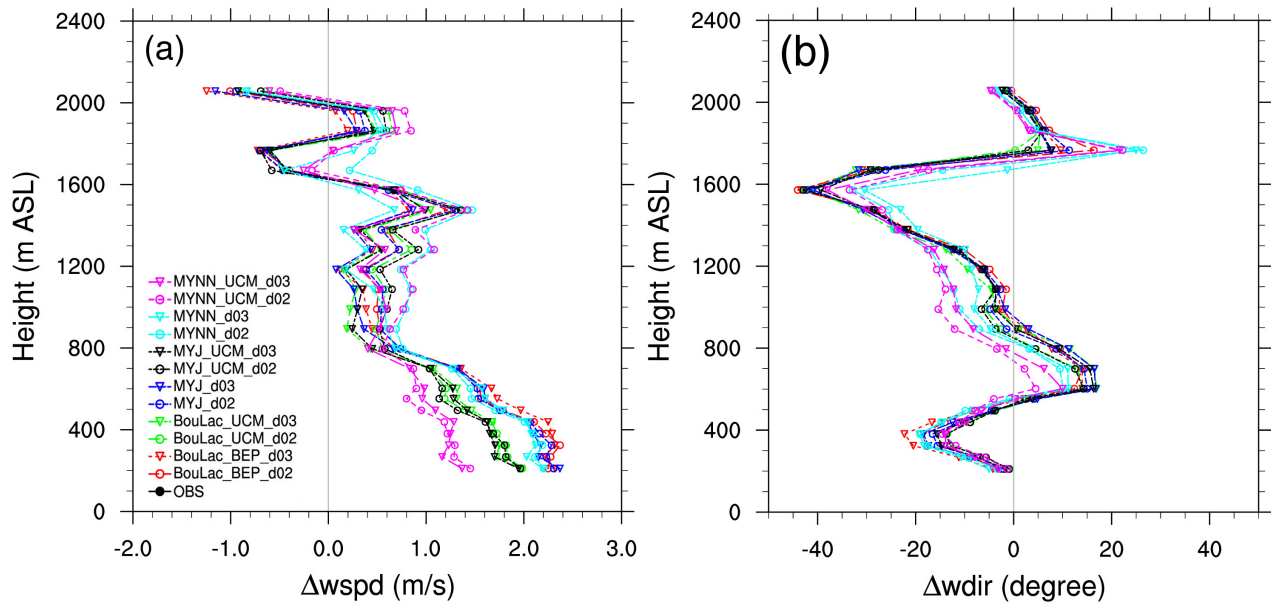
Figure 5. Average differences of wind profiles between the simulations and observations (model - wind radar profiler) at the Los Angeles International Airport (LAX). (a) The difference for wind speed (unit: \text{ms}^{-1} ); (b) for wind direction (unit: degree). Note that these results are for daytime 1100 - 1700 PST only.
