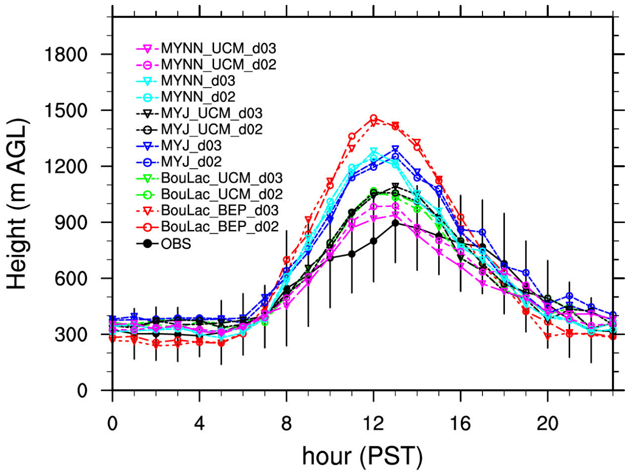
Figure 4. Average diurnal variation of the ceilometer-measured and modelled PBL heights at California Institute of Technology (Caltech) in Pasadena, CA during 15 May through 15 June 2010. Error bars indicate standard deviations of the means of the ceilometer measurement.
