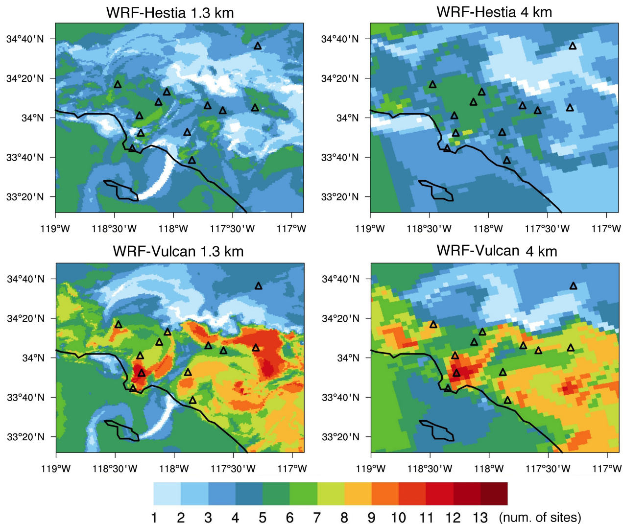
Figure 14. Composite maps of spatial correlation ( R in Figure 12 and 13) for the 1.3-km WRF-Hestia, 1.3-km WRF-Vulcan, 4-km WRF-Hestia, and 4-km WRF-Vulcan runs. Each composite map was constructed by determining the number of the observation sites for which |R| is greater than 0.46 at each grid cell. |R| = 0.46 is the critical value at the significance level of 0.01 of t -test. Specifically, white cells indicate that no sites are correlated well at the location; dark red cells indicate that over 13 sites have good correlation at the location. The SCI and Dryden sites are not shown on these maps.
