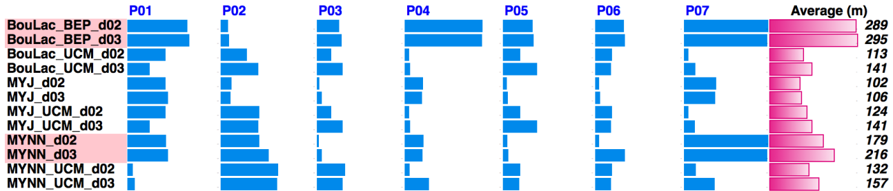
Figure 3. Absolute difference between the aircraft-determined and modelled PBL height for each profile: P01, P02, ..., and P07 (blue bars). The pink bars in the last column represent the averaged bias over all of the profiles for each configuration. Note that the shorter the bar, the better agreement of the model with the observations.
