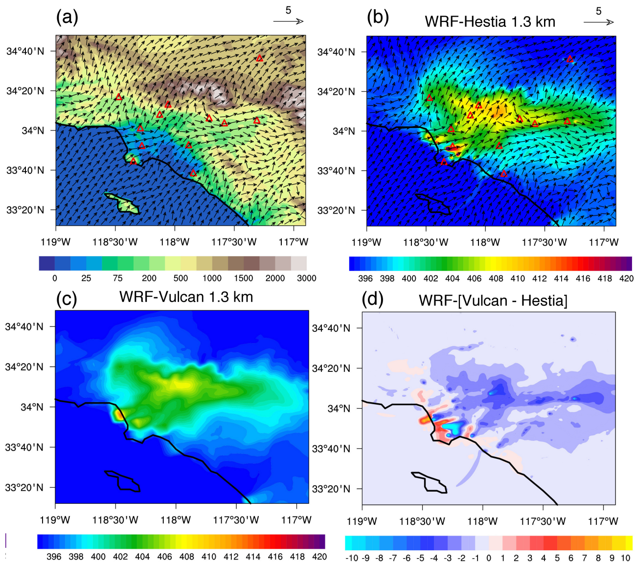
Figure 11. (a and b) The first empirical orthogonal function (EOF 1) for the surface wind pattern (black arrows) simulated by MYNN_UCM_d03 at 1400 PST during CalNex-LA. EOF 1 accounts for 48.1 % of the variance in the average winds. Contours: (a) terrain height (unit: m); (b) the modelled surface CO 2 concentration (unit: ppm) from the 1.3-km WRF-Hestia run. The red triangles indicate the locations of the GHG measurement sites. (c) The modelled CO 2 concentrations from the 1.3-km WRF-Vulcan run (unit: ppm). (d) The difference in the modelled CO 2 concentrations between the 1.3-km WRF-Vulcan and WRF-Hestia runs (unit: ppm).
