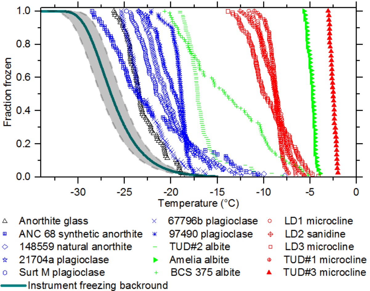
6 Figure 2: Droplet fraction frozen as a function of temperature for 1 wt% suspensions of 7 ground powders of various feldspar samples. The K-feldspars are coloured red, the 8 plagioclase feldspars are coloured blue, the albites are coloured green and the feldspar glass 9 is coloured black. A fit to the background freezing of pure MilliQ water in the \mu l-NIPI 10 instrument used by Umo et al. (2015) is also included. The shaded area around this fit shows 11 95% confidence intervals for the fit. It can be seen that all the feldspar samples tested 12 nucleate ice more efficiently than the background freezing of the instrument.
