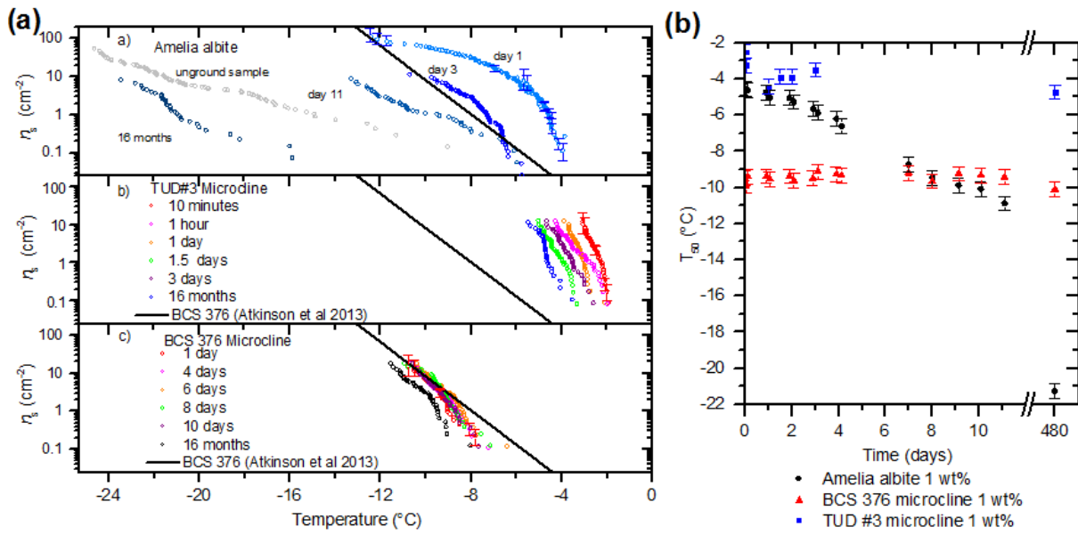
2 Figure 4 (a) The dependence of n_s on time spent in water for three feldspar samples. The time 3 periods indicate how long samples were left in contact with water. Fresh samples were tested 4 minutes after preparation of suspensions. Note that ice nucleation temperatures of BCS 376 5 are almost the same after 16 months in water while those of Amelia albite decreases by 6 around 16°C. TUD #3 microcline loses activity quickly in the first couple of days of exposure 7 to water but total decrease in nucleation temperatures after 16 months is only around 2°C. (b) 8 Median freezing temperature against time left in suspension for BCS 376 microcline, TUD#3 9 microcline and Amelia albite.
