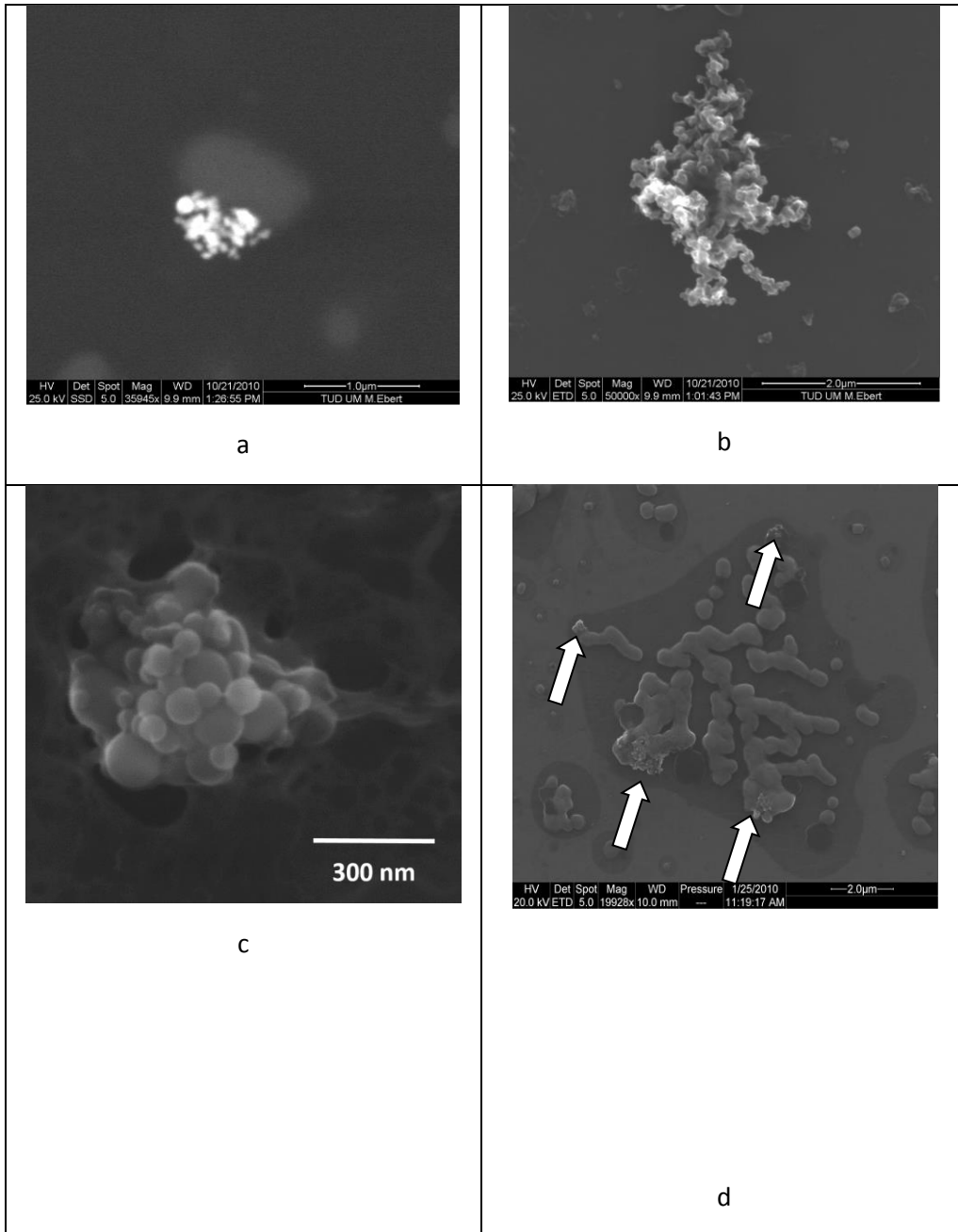
Figure 6: Secondary electron images of refractory particles in the fine fraction. a) Lead rich agglomerate (bright) within a secondary particle, b) soot particle, c) agglomerate of spherical silicate particles, and d) soot inclusions (marked by arrows) within volatile material.
