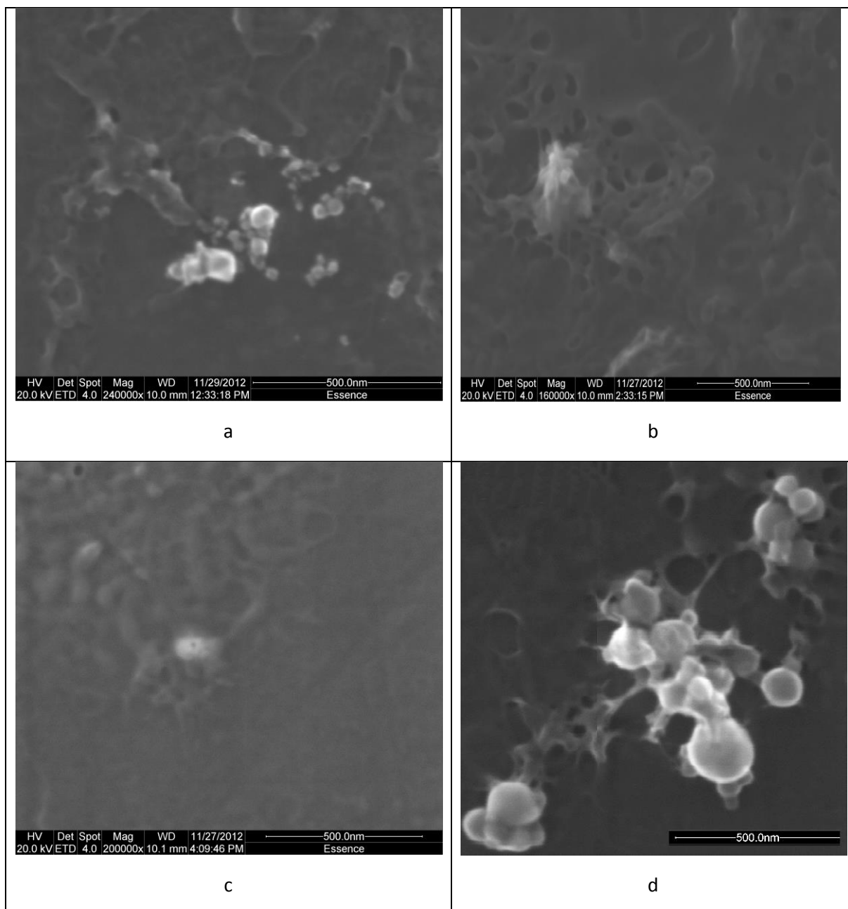
Figure 7: Secondary electron images of refractory particles in the fine fraction of ESSenCe samples. a) Aluminum oxide spheres (AOS); b) Fe-rich particles; c) Pb-rich particles; d) Mg-rich silicates.
