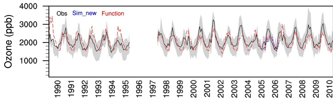
Fig. 2. O 3 trend in the top layers (pressure < 100 hPa) in the Arctic (latitude > 75°N)
