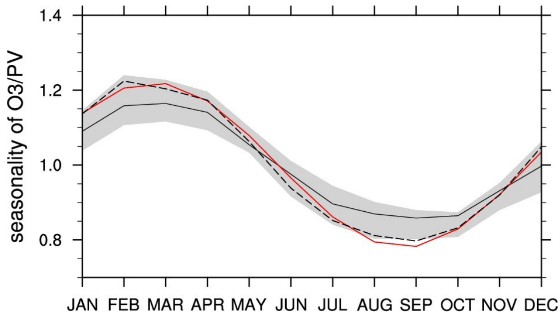
Fig. 1. Seasonality of O 3 /P V (Annual mean= 1, black solid line=observed mean at all sites, grey, black dash line= observed mean at sites at latitudes north of 40N, red line = fitted by function)
