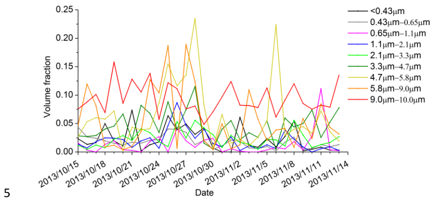
Fig. 5 Time series of the volume fraction of EC for different size segments during the observation period
