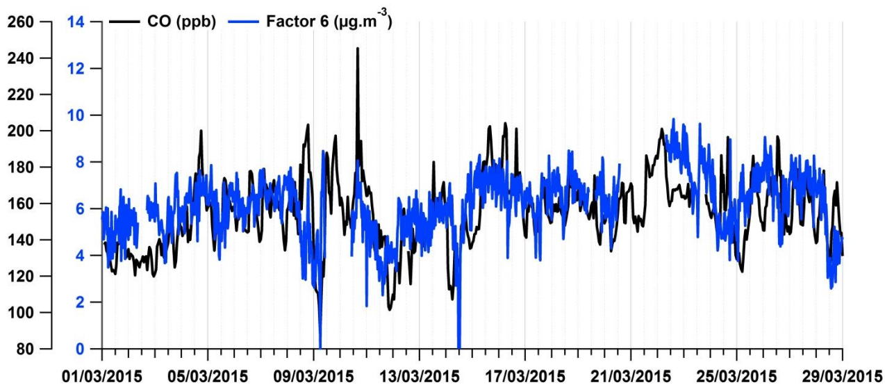
Figure 14: Time series of the VOCs factor 6 contribution (blue line) and CO (dark line).
