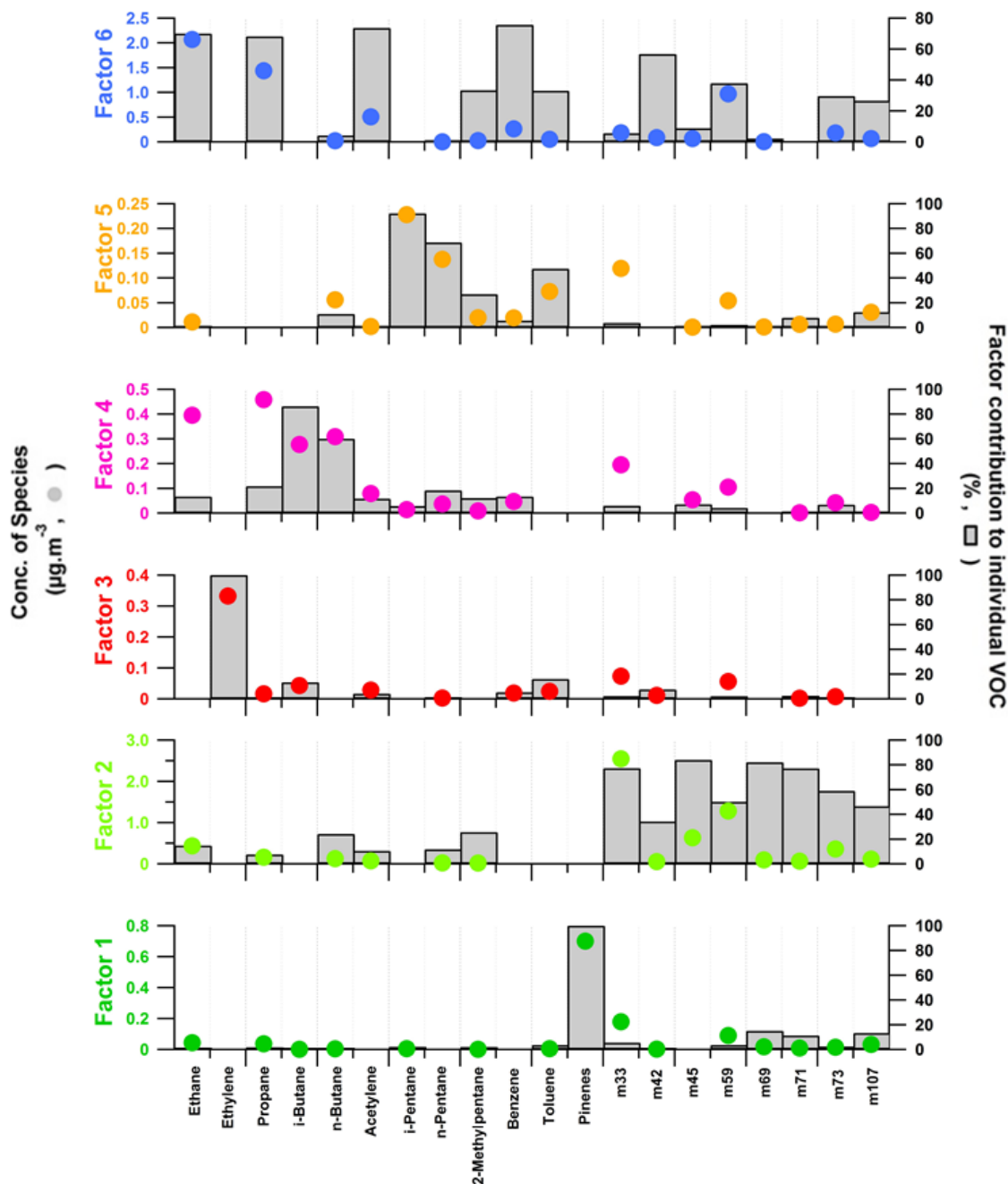
Figure 7: Chemical profiles of the 6-factor PMF solution (20 VOCs). The contribution of the factor to each species ( \mu\text{g. m}^{-3} ) and the percent of each species apportioned to the factor are displayed as a grey bar and a color circle, respectively. Factor 1 - biogenic source 1; factor 2 - biogenic source 2; factor 3 – short-lived combustion source; factor 4 – evaporative sources; factor 5 – industrial and evaporative sources; factor 6 – regional background.
