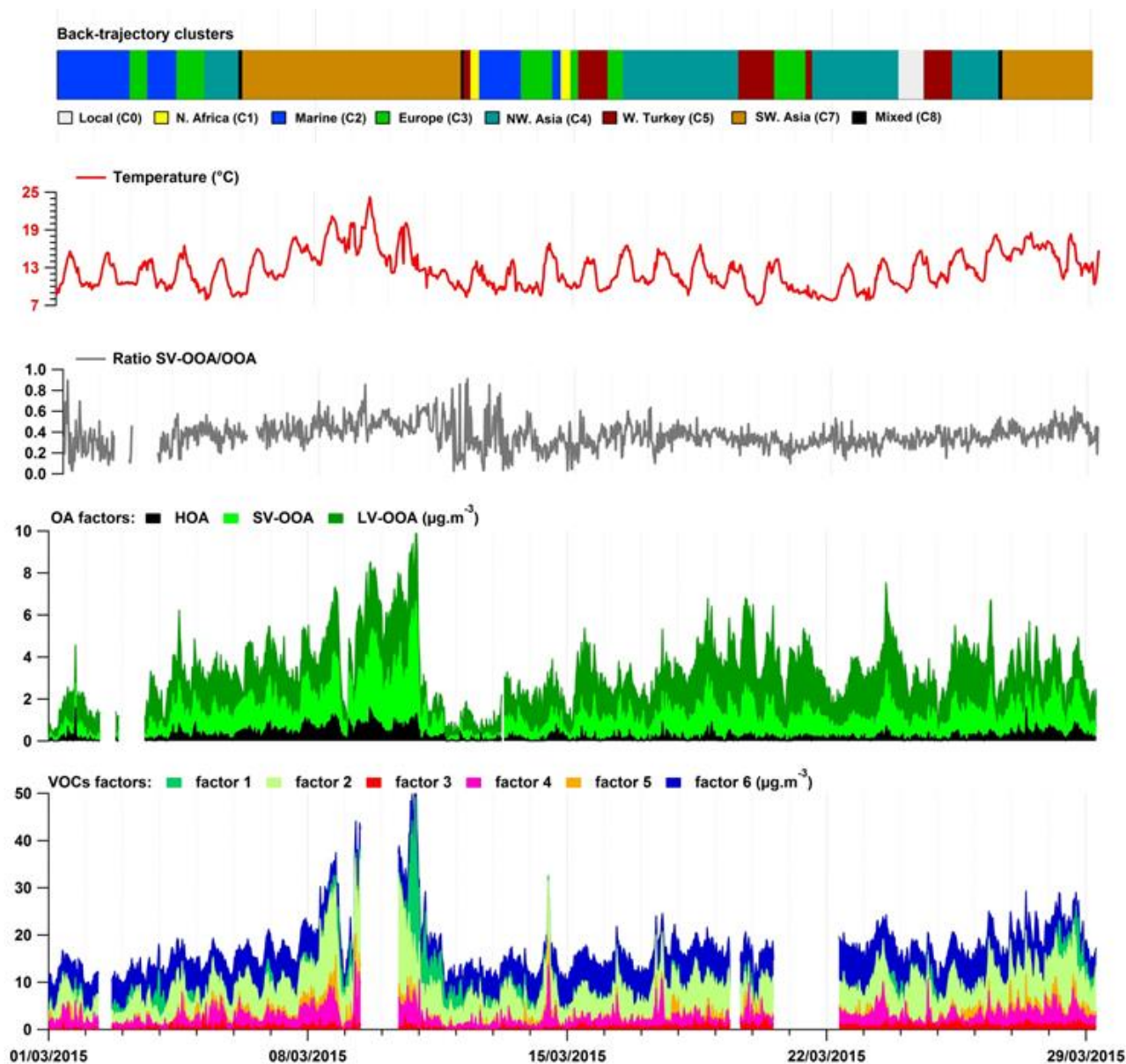
Figure 17: Accumulated time series of OA and VOCs factor contribution, time series of temperature and air masses origin (C: cluster). VOCs factors: factor 1 - biogenic source 1; factor 2 - biogenic source 2; factor 3 – short-lived combustion source; factor 4 – evaporative sources; factor 5 – industrial and evaporative sources; factor 6 – regional background. OA factors: HOA - hydrogen-like OA; SV-OOA – semi-volatile oxygen-like OA; LV-OOA – low-volatile oxygen-like OA.
