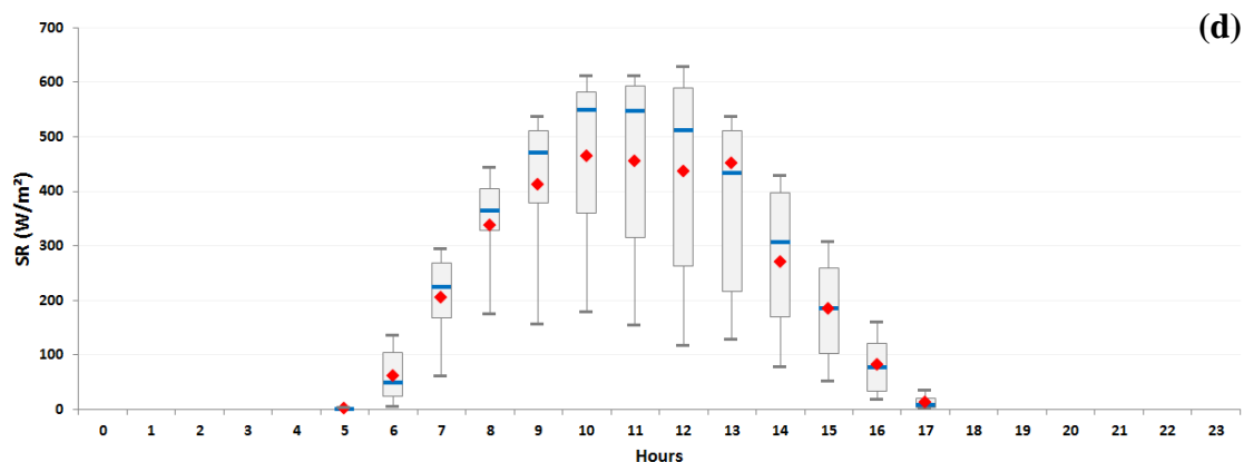
5 Figure 9: Diel variation of the VOCs factor contribution (A and B), temperature and solar radiation (C and D) represented by hourly box plots. Blue solid line represents the median value, the red marker represents the mean value and the box shows the InterQuartile Range (IQR). The bottom and the top of box depict the first and the third quartiles (i. e. Q1 and Q3). The ends of the whiskers correspond to first and the ninth deciles (i. e. D1 and D9). Time is given as local time.
