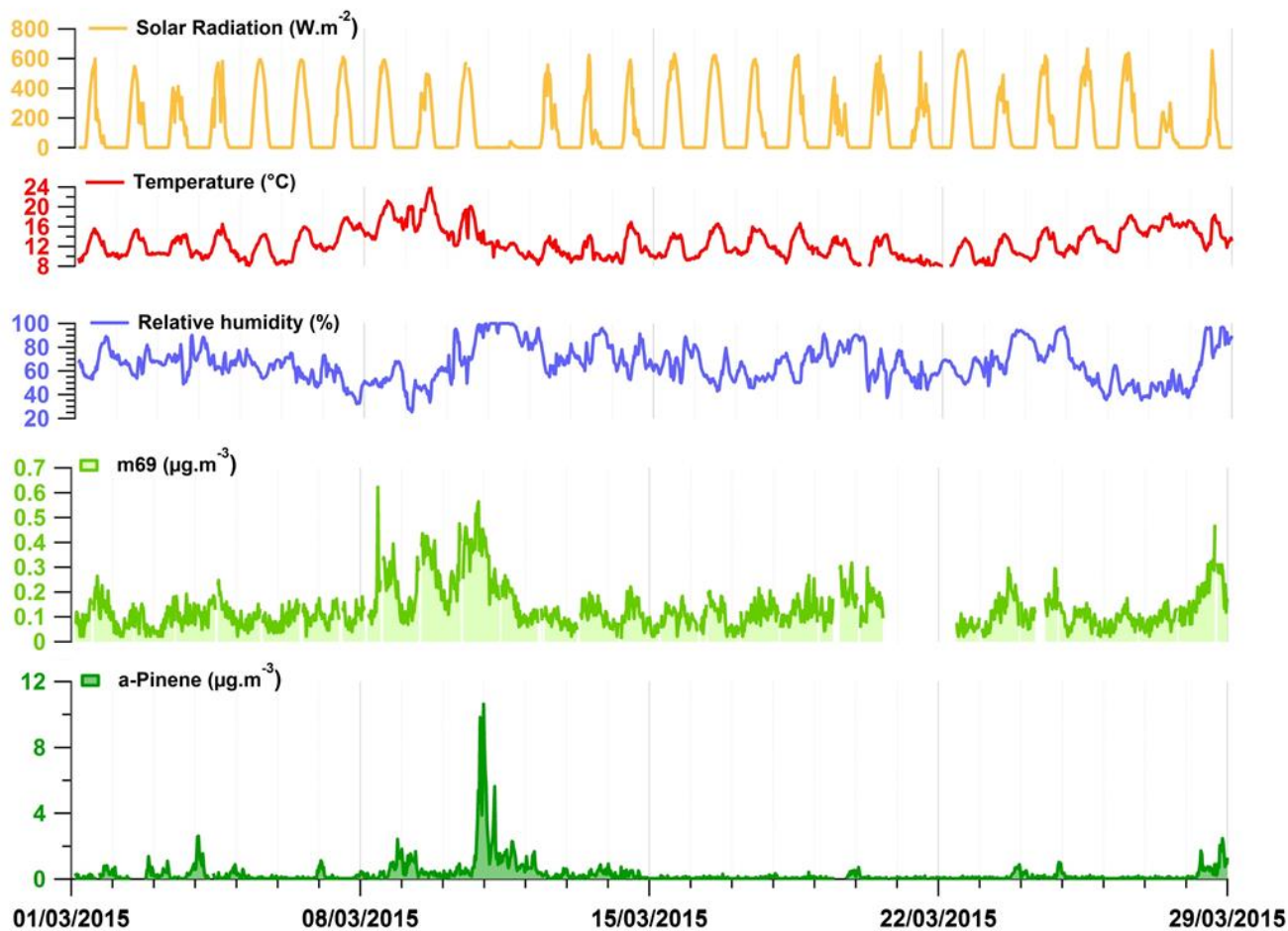
Figure 5: Time series of a selection of anthropogenic VOCs (isoprene and \alpha -pinene – green lines) in comparison with meteorological parameters (solar radiation, temperature and relative humidity; displayed as orange, red and blue lines, respectively).
