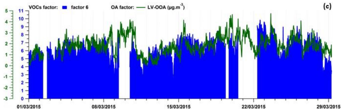
5 Figure 19: Time series of OA and VOCs factor contributions of March 2015 (figures A and C) or of selected days of the intensive field campaign (figures B1, B2, B3) to point out co-variations and confirm average daily variations presented in figure S9 in the supplement. VOCs factors: factor 1 - biogenic source 1; factor 2 - biogenic source 2; factor 3 – short-lived combustion source; factor 4 – evaporative sources; factor 5 – industrial and evaporative sources; factor 6 – regional background. OA factors: HOA - hydrogen-like OA; SV-OOA – semi-volatile oxygen-like OA; LV-OOA – low-volatile oxygen-like OA.
