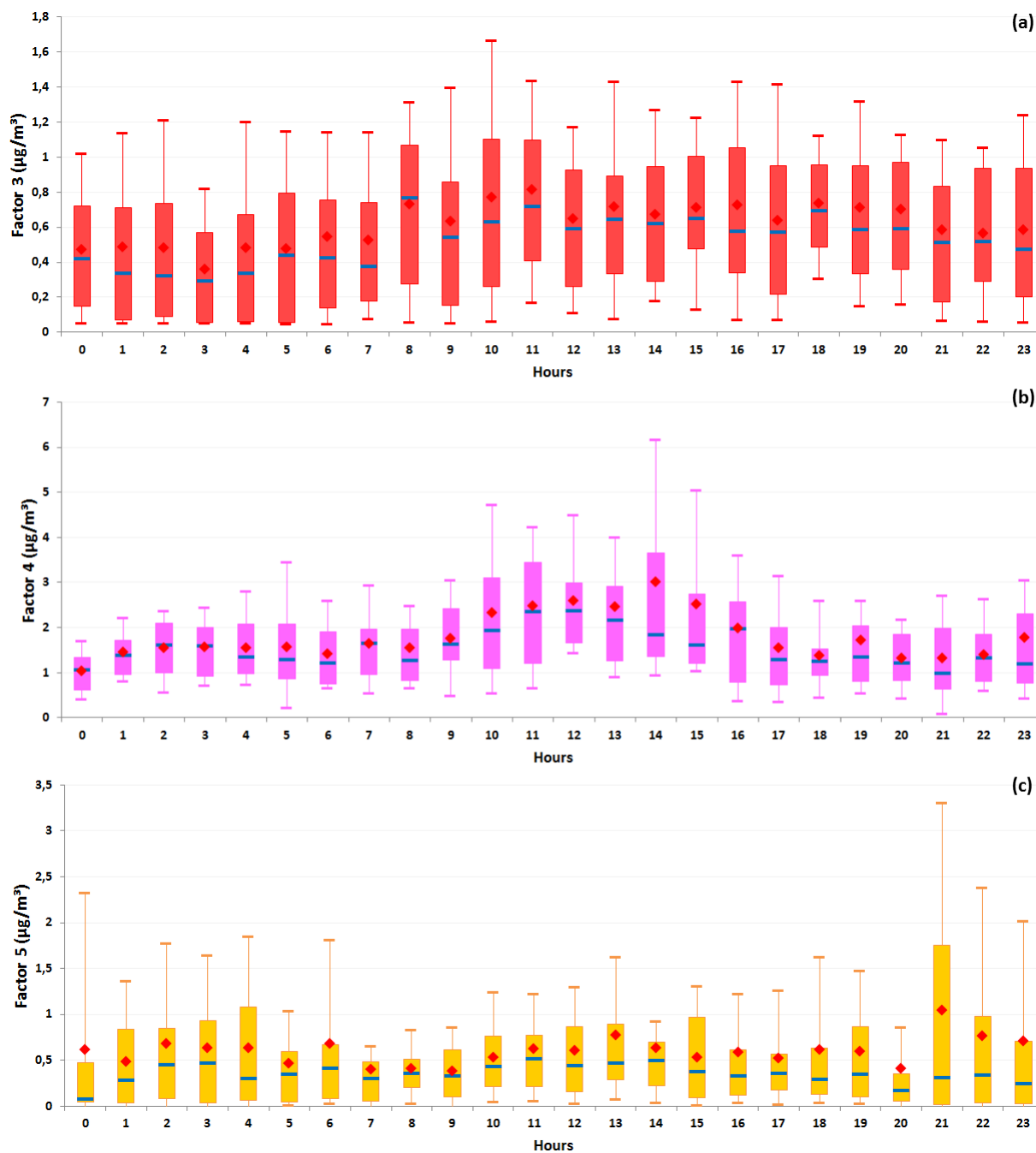
5 Figure 12: Diel variation of the factor contributions (A, B and C) represented by hourly box plots. Diurnal profiles do not include contributions obtained when the site was under the influence of air masses categorized in cluster 7. Blue solid line represents the median contribution, the red marker represents the mean contribution and the box shows the InterQuartile Range (IQR). The bottom and the top of box depict the first and the third quartiles (i. e. Q1 and Q3). The ends of the whiskers correspond to first and the ninth deciles (i. e. D1 and D9). Time is given as local time.
