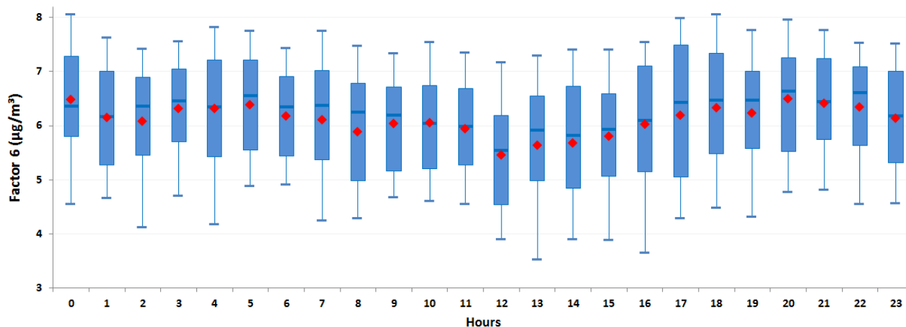
5 Figure 15: Diel variation of the VOCs factor 6 contributions represented by hourly box plots. Blue solid line represents the median contribution, the red marker represents the mean contribution and the box shows the InterQuartile Range (IQR). The bottom and the top of box depict the first and the third quartiles (i. e. Q1 and Q3). The ends of the whiskers correspond to first and the ninth deciles (i. e. D1 and D9). Time is given as local time.
