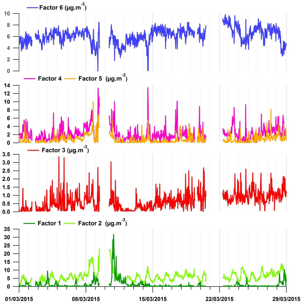
Figure 8: Time series of VOCs factor contributions ( \mu\text{g. m}^{-3} ). Factor 1 - biogenic source 1; factor 2 - biogenic source 2; factor 3 – short-lived combustion source; factor 4 – evaporative sources; factor 5 – industrial and evaporative sources; factor 6 – regional background.
