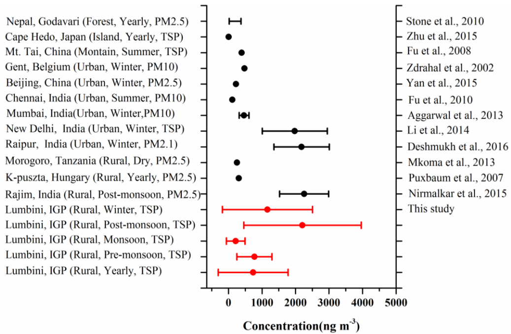
Fig. 5. Comparison of levoglucosan concentrations in Lumbini with other sites in different locations worldwide.
