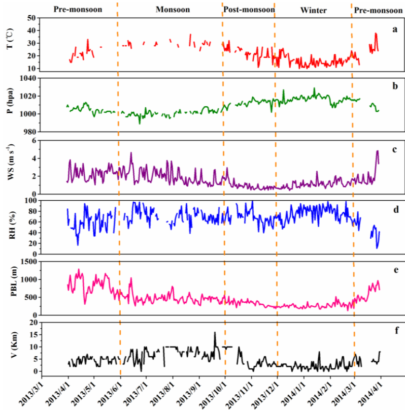
790 Fig. 2. Time series of ambient temperature (T), atmospheric pressure (P), wind speed (WS), relative humidity (RH), planetary boundary layer (PBL), and visibility (V) at Lumbini from April 2013 to March 2014.
