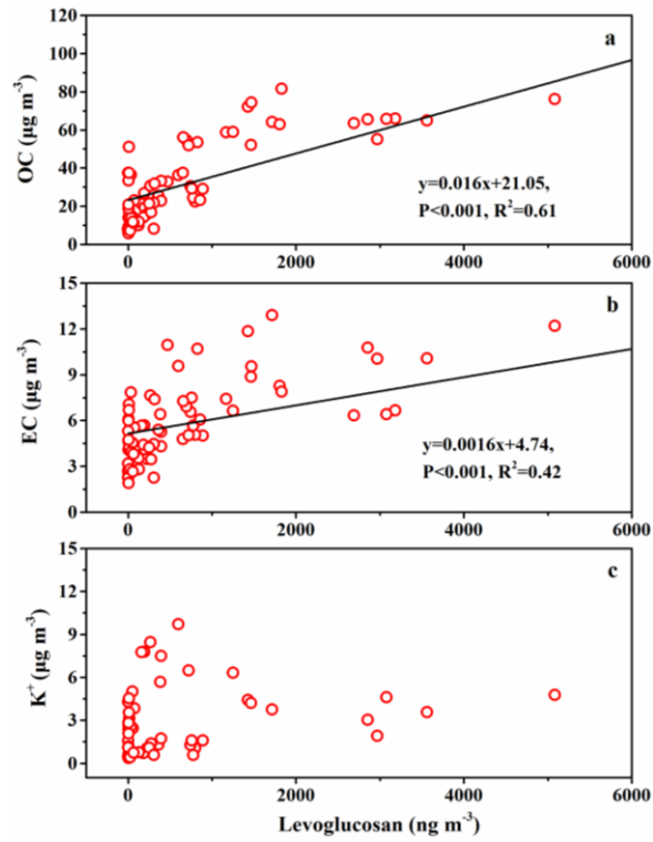
805 Fig. 6. Correlations between (a) levoglucosan and OC, (b) levoglucosan and EC, and (c) levoglucosan and K + during the whole year.
