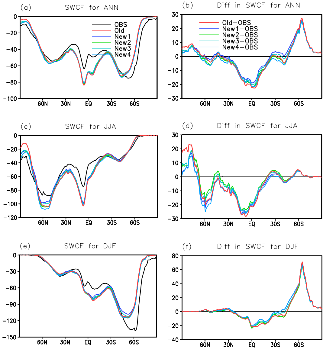
Figure 2. Annual, JJA and DJF zonal mean of shortwave cloud radiative forcing (SWCF, W m^{-2} ) derived from CAM5.1 (a, c and e) and the CERES-EBAF observations (OBS), and their difference between OBS and Old, as well as News (b, d and f).
