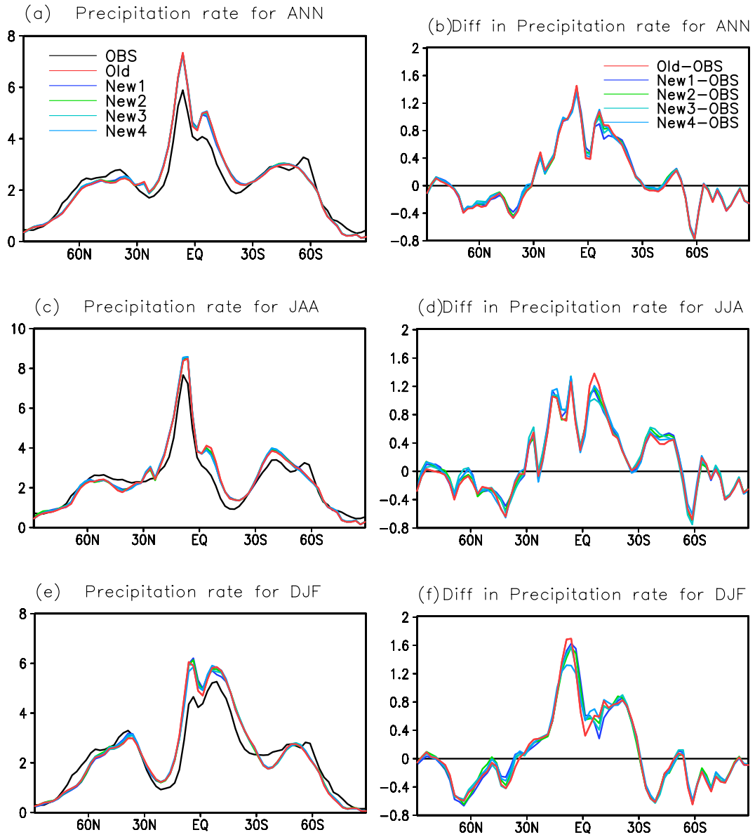
Figure 4. Annual, JJA and DJF zonal mean of the total precipitation rate (mm day -1 ) derived from CAM5.1 (a, c and e) and the GPCP observations (OBS), and their corresponding difference between OBS and Old, as well as News (b, d and f).
