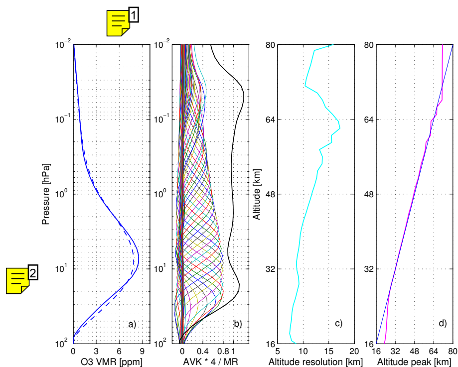
Figure 3. a) Example of a daily mean retrieved ozone profile (solid line) together with the a priori profile used for the inversion (dashed line). b) The corresponding averaging kernels (colour lines) and the measurement response (black line). c) Width of the averaging kernels as a measure of vertical resolution. d) Altitude of the averaging kernels peak.
