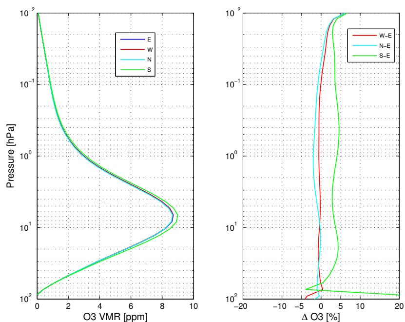
Figure 4. Comparison of ozone profiles in 4 directions of view. Each profile corresponds to the whole campaign mean of daily mean profiles. The right plot shows the relative differences respect the East profile.
