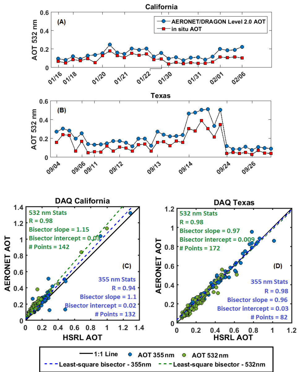
Figure 10. (top) AERONET and in situ AOT measurements during DAQ CA (A) and TX (B). In situ values were obtained by vertical integration of the ambient extinction profile. (bottom) Comparison of AOT measurements at 355 and 532 nm measured with HSRL-2 and AERONET/DRAGON sunphotometers during DAQ California (C) and DAQ Texas (D). Measurements from AERONET were calculated from level 2.0 measurements of AOT at 340 nm and 500 nm, corrected to 355 and 532 nm using Ångström exponents calculated between 340 and 440 nm, and 440 and 675 nm, respectively. Only measurements obtained within a radius of 2.5 km and 10 minutes from each other were considered.
