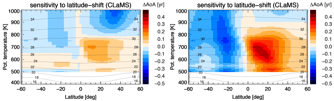
Figure B1. Left panel: Zonal mean AoA distribution of period I from CLaMS shifted by the shift profile plus 1\text{-}\sigma uncertainty (reducing the shift below 800 K); right panel: same as left, but shifted by the shift profile minus 1\text{-}\sigma uncertainty (increasing the shift below 800 K).
