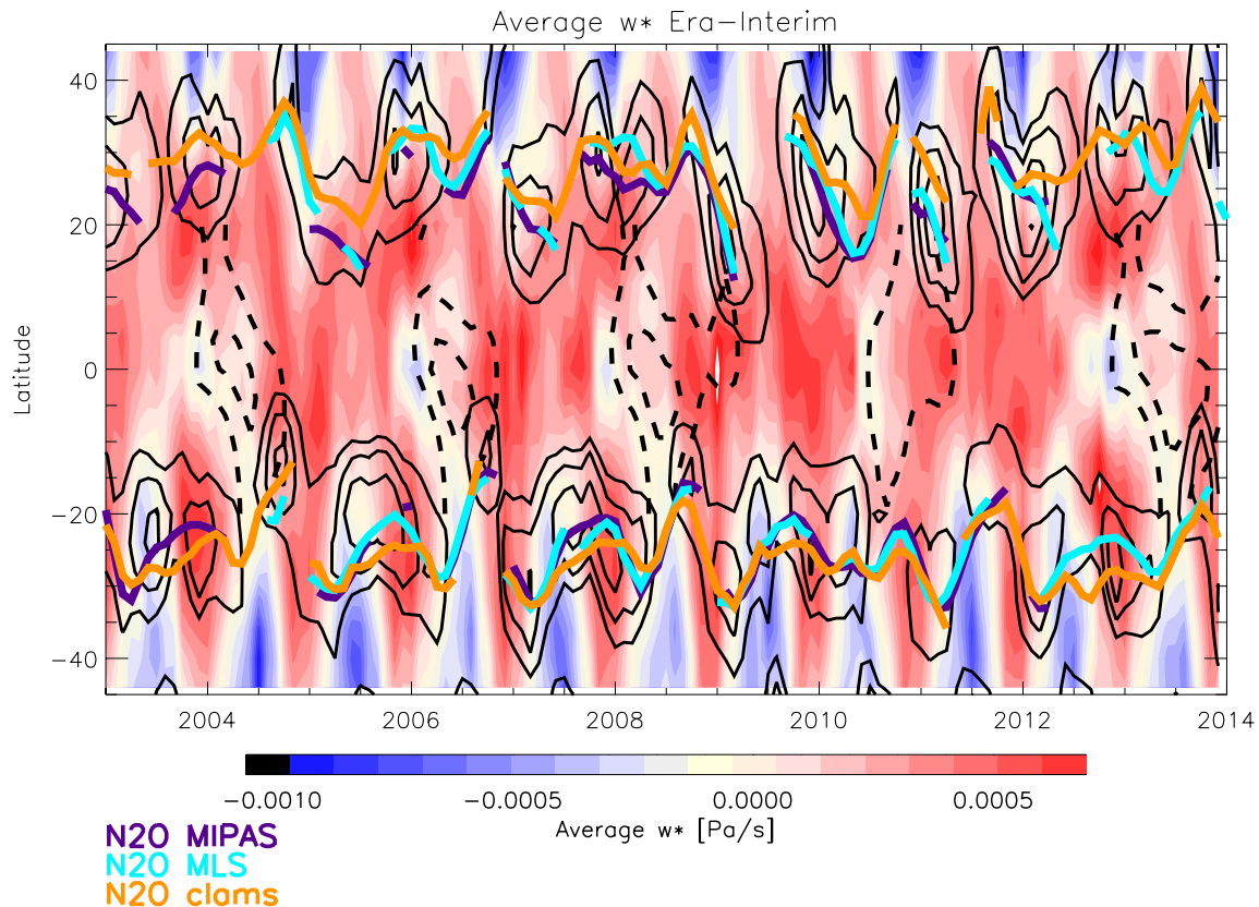
Figure 3. Positions of the subtropical transport barriers over time at 600K compared to other dynamical quantities providing a measure for the position of the tropical pipe: the purple, turquoise and orange solid lines provide the positions of the subtropical transport barriers from MIPAS, MLS, and CLAMS data, respectively, derived with the method of Palazzi et al. (2011); the color coding indicates the values of \bar{w}^* (see color bar); the latitude regions of maximum meridional tracer gradients are indicated as black contour lines. Black dashed lines enclose the regions of positive zonal-mean zonal wind (QBO positive phases).
