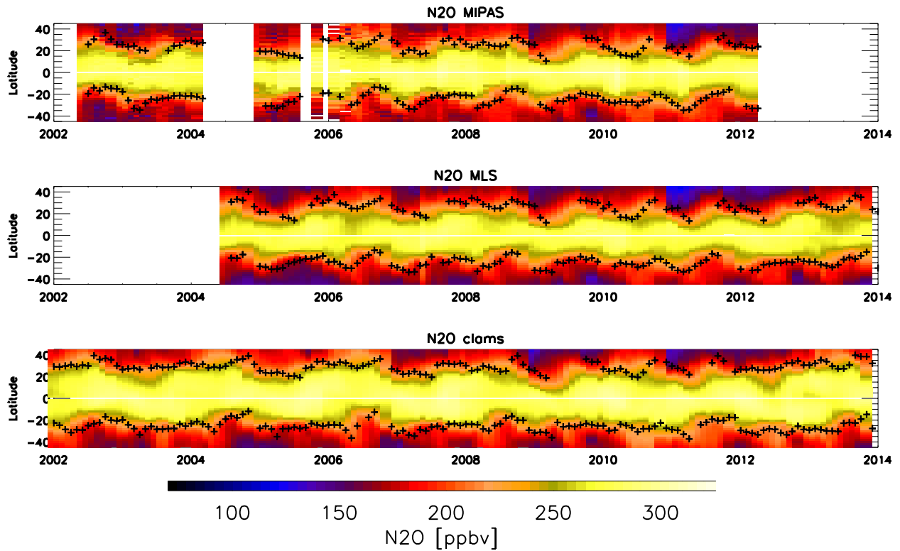
Figure 1. Time series of zonal \text{N}_2\text{O} distributions at the 600 K potential temperature level from MIPAS observations (top panel), MLS observations (middle panel), and CLaMS model simulations driven by ERA-Interim reanalyses (bottom panel). The black crosses indicate the positions of the subtropical transport barriers derived with the method by Palazzi et al. (2011). Gaps in the time series of transport barrier positions appear where the method for determining the positions failed.
