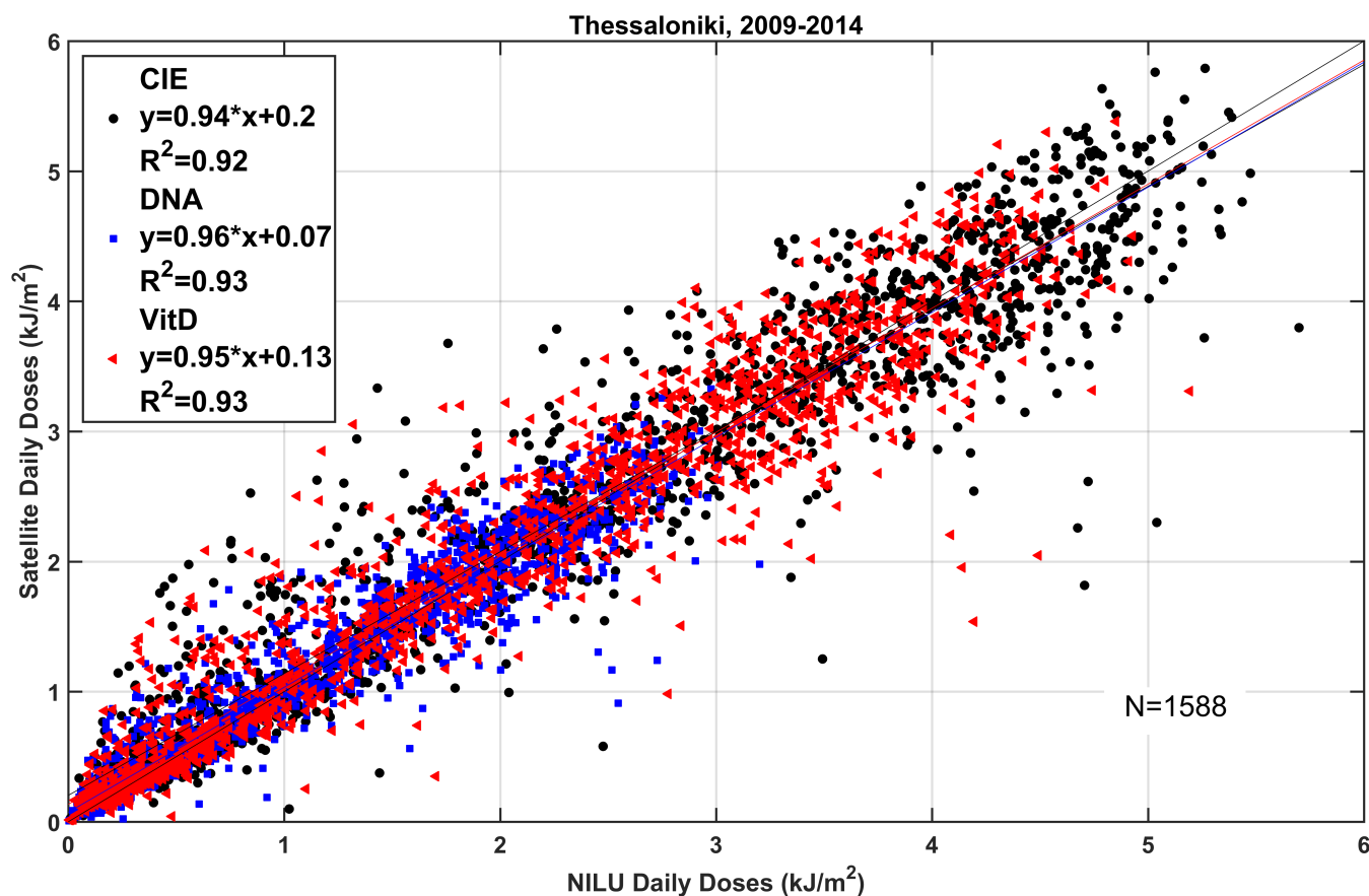
Figure 7. Scatter plot of daily UV dose values provided by the joint SCIA/GOME2A UV products (y-axis) and NILU103 (x-axis) in \text{kJ}/\text{m}^2 .
