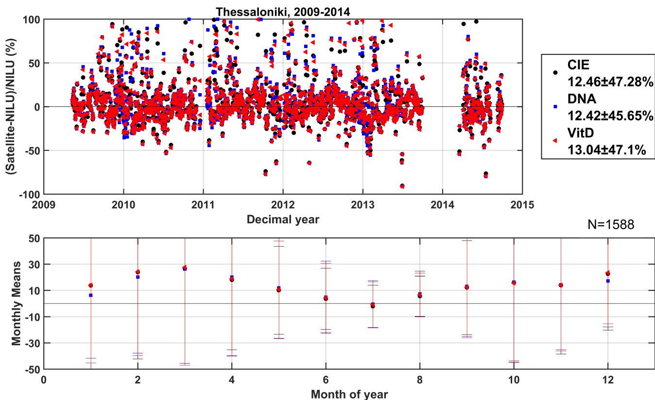
Figure 6. Time series of the relative percentage differences between the SCIAMACHY/GOME2A and NILU-UV effective daily doses (upper level) and the seasonality of the differences based on the average month along with the 1-sigma error bars (lower level).
