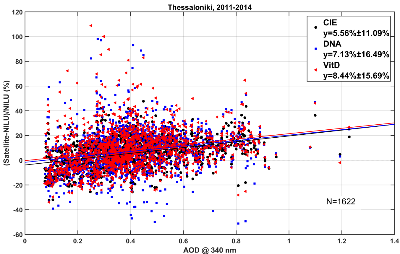
Figure 10. Relative differences of satellite-based and ground-based UV daily doses as a function of AOD at 340 nm for cloudless days at Thessaloniki in the period 2011-2014. The statistics are provided in the form of mean and standard deviation of the differences.
