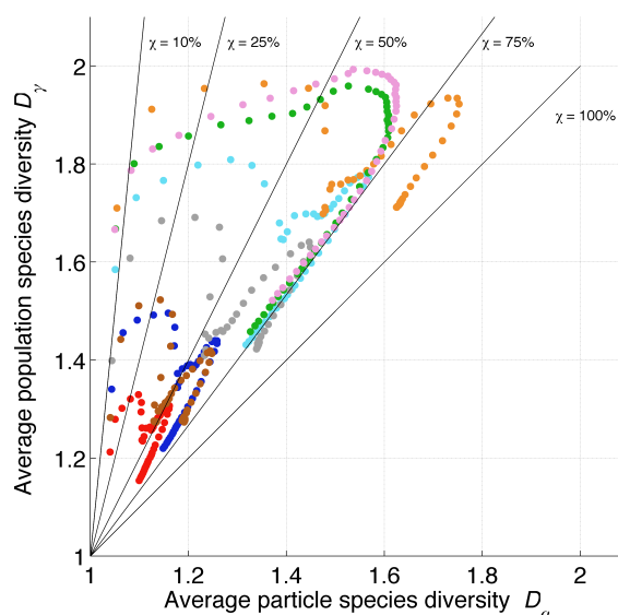
Figure 2. Mixing state diagram for the 384 populations in \mathbb{P} . The colors indicate the Ching et al. (2016a) scenario from which the populations were sampled: B100-E100-G100 (light blue), B100-E100-G100 (orange), B100-E25-G100 (blue), B100-E25-G100 (grey), B100-E2.5-G100 (red), B100-E2.5-G100 (brown), B100-E100-G50 (green) and B100-E100-G25 (pink). The abbreviations of the scenarios follow Ching et al. (2016a), “B” indicates the level of background particle concentration (100% and 10% of the base case scenario), “E” indicates the level of the black carbon emission rate (100%, 25%, and 2.5% of the base case scenario) and “G” indicates the level of gas emission rate (100%, 50%, and 25% of the base case scenario).
