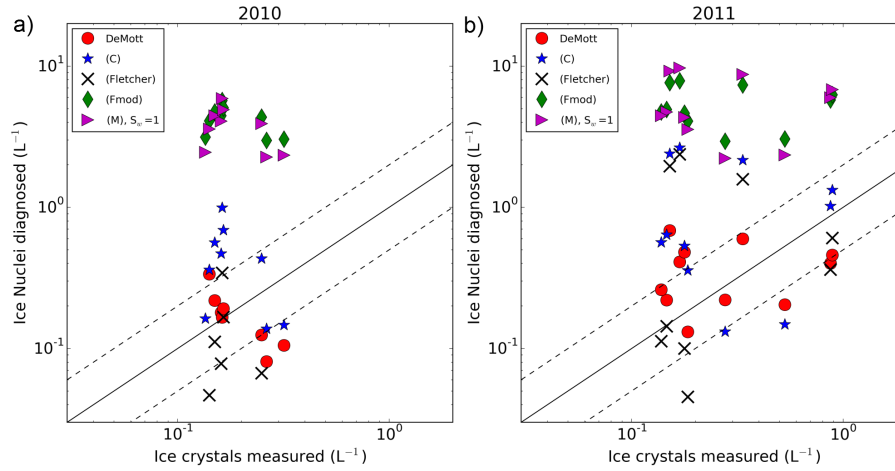
Figure 14. Predicted INP number densities versus observed number densities of crystals (flights averages) for various INP parameterisations for (a) 2010, and (b) 2011. The solid lines corresponds to the one-to-one line, and the dashed lines corresponds to a factor of two difference between y and x axes. See Table 3 for the references of the various INP parameterisations.
