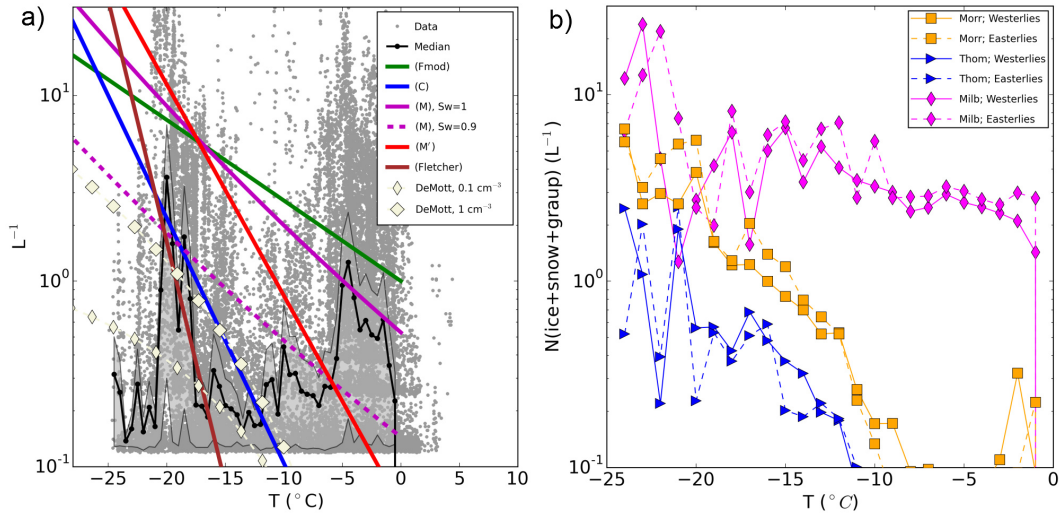
Figure 13. (a) Ice crystals measurements data points as a function of the temperature (grey) with their median per 0.5°C bins (black solid line), along with the absolute median deviation in shaded grey. The labelled INP parameterisations used by the different cloud schemes (Table 3) are overplotted. DeMott refers to DeMott et al. (2010)’s INP parameterisation (see text for details). (b) Same as (a) for the Median of the total number concentrations of icy hydrometeors in the same transects used in Figure 5 for both cases, the westerly case (solid lines), and the easterly case (dashed lines).
