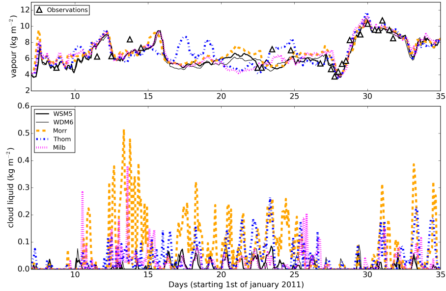
Figure 2. (Top) Time series of column density of water vapour ( \text{kg m}^{-2} ) for the different simulations computed in the model gridbox corresponding to the AWS14 location, in 2011, along with the radiosonde measurements from the field camp (described in K15, see their Figure 7). (Bottom) Time series of the column density of the cloud liquid ( \text{kg m}^{-2} ) for the different simulations.
