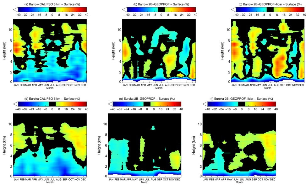
Figure 3: Cloud fraction vertical distribution difference for 2006-2010 from (a) CALIPSO 5km, (b) 2B-GEOPROF, and (c) 2B-GEOPROF-lidar and surface observations at Barrow; and from (d) CALIPSO 5 km, (e) 2B-GEOPROF, and (f) 2B-GEOPROF-lidar and surface observations at Eureka.
