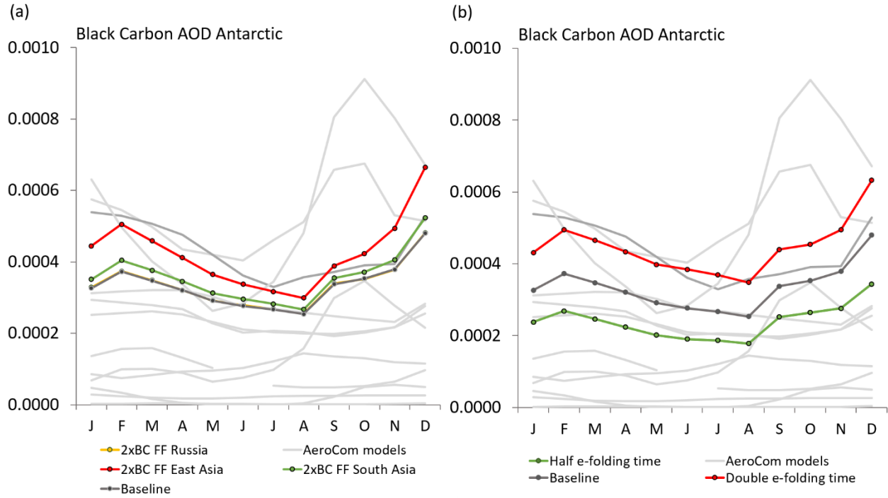
Figure S1: Antarctic mean seasonal cycle of (total) BC AOD for simulations with GISS modelE (in colors) compared to the AeroCom models (in light grey). The darker grey AeroCom model is the GISS modelE AeroCom run. (a) shows emission perturbations for a doubling of BC emissions (fossil fuel and biofuel) in South Asia (green), East Asia (red), and Russia (yellow). (b) shows double (red) and half (green) of the e-folding time from hydrophobic to hydrophilic BC.
