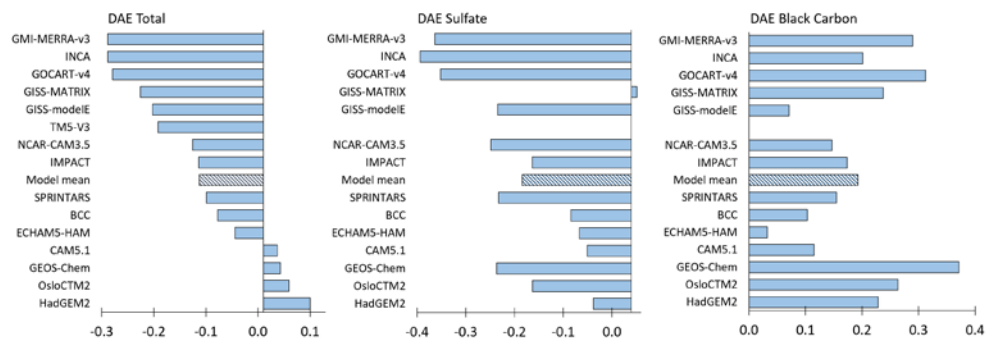
5 Figure 15: Arctic annual mean DAE (in W m^{-2} ) for the AeroCom phase II models, total (left), sulfate (middle), BC FF (right). The striped bar is the model mean. TM5-V3 have reported total only.
