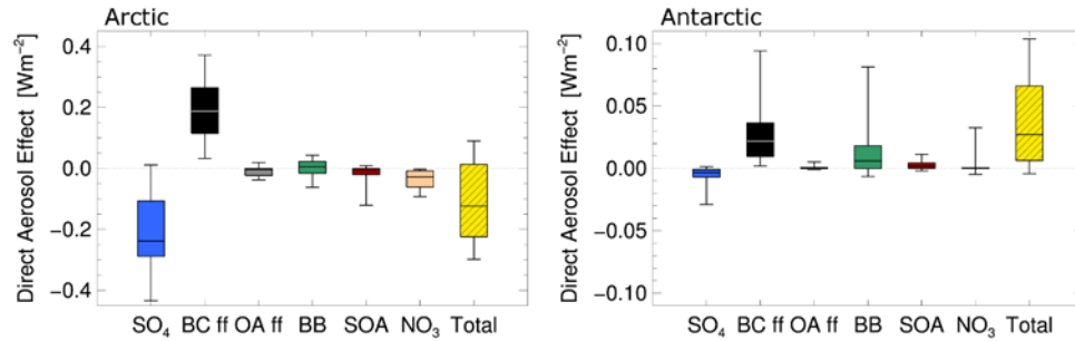
5 Figure 12: Annual mean multi-model DAE (in \text{W m}^{-2} ) averaged over the Arctic ( 60^{\circ}\text{N} - 90^{\circ}\text{N} ) (left) and the Antarctic ( 70^{\circ}\text{S} - 90^{\circ}\text{S} ) (right), for the individual components (sulfate, BC FF, OA FF, BB, SOA, and nitrate) and the total aerosol. The bottom and top of each box are the first and third ( 25^{\text{th}}/75^{\text{th}} ) quartiles, and the band inside the box is the model-median. The whiskers represent the minimum and maximum of the model range. Note the different vertical axis.
