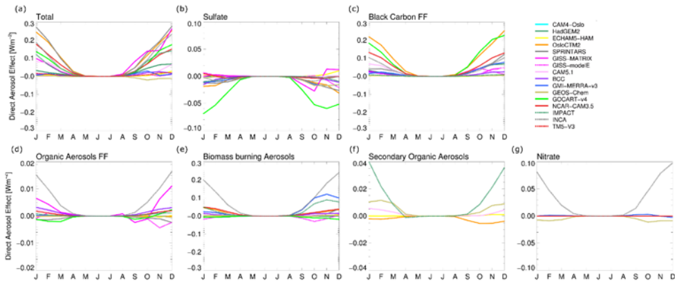
5 Figure 17: Antarctic mean ( 70^{\circ}\text{S} - 90^{\circ}\text{S} ) seasonal cycle of (a) the total DAE and the DAE for (b) sulfate, (c) BC FF, (d) OA FF, (e) BB, (f) SOA, and (g) nitrate. Note the different axes.
