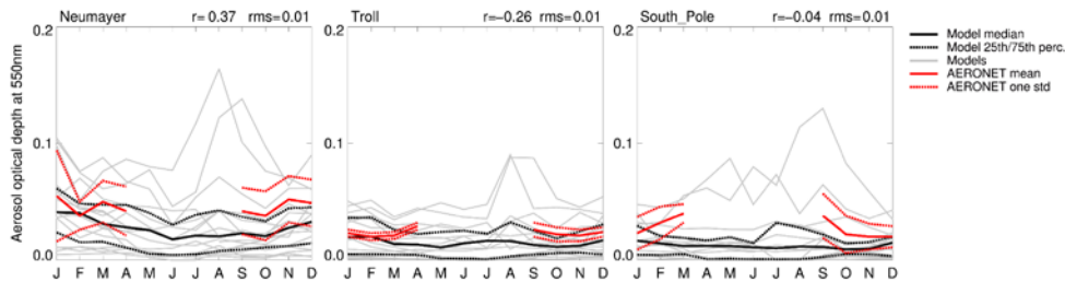
5 Figure 7: As Fig. 2, but for three Antarctic sites: Neumayer 70^{\circ}\text{ S}, 8^{\circ}\text{ W} (left), Troll 72^{\circ}\text{ S}, 2^{\circ}\text{ E} (middle), and South Pole 90^{\circ}\text{ S}, 0^{\circ}\text{ E} (right), with values from Tomasi et al. (2015).
