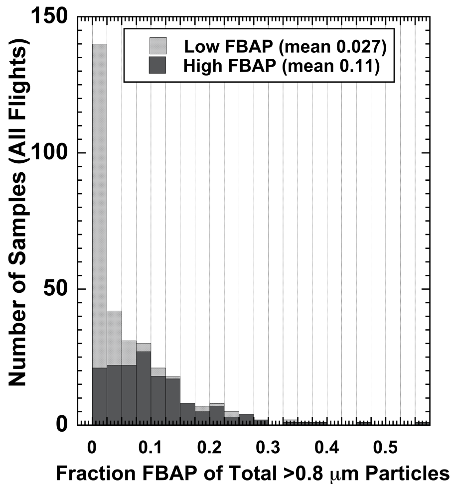
Figure 6. Ratio of FBAP number concentration to total particle number concentration in the 0.8-12 μm size range, using expected low and high bounds as discussed in the text. Histograms of 200 second average values for WIBS-4A samples on all five flights are plotted. Legend shows the mean fraction for each FBAP category.
