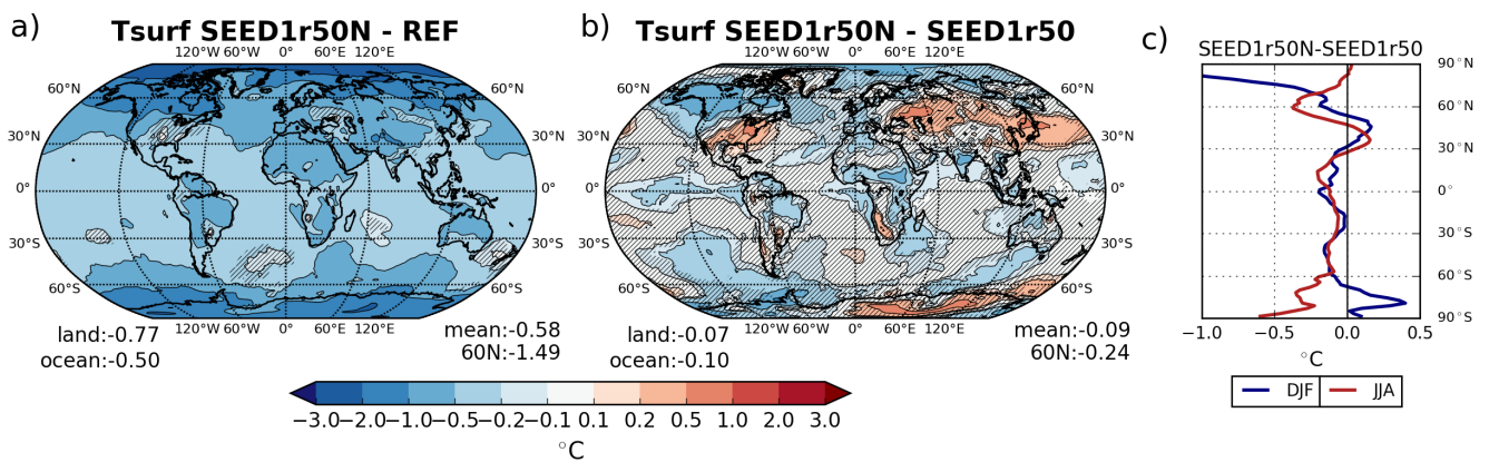
Figure 8. Annually averaged anomalies of surface temperature (T surf ) for the SEED1r50N simulation with respect to REF (a) or SEED1r50 (b). The hatching is applied for anomalies not significant at the 95% confidence level. Panel c) shows the respective annual zonal average anomalies of SEED1r50N with respect to SEED1r50 for DJF (blue) and JJA (red). All simulations are performed in the MLO setup.
