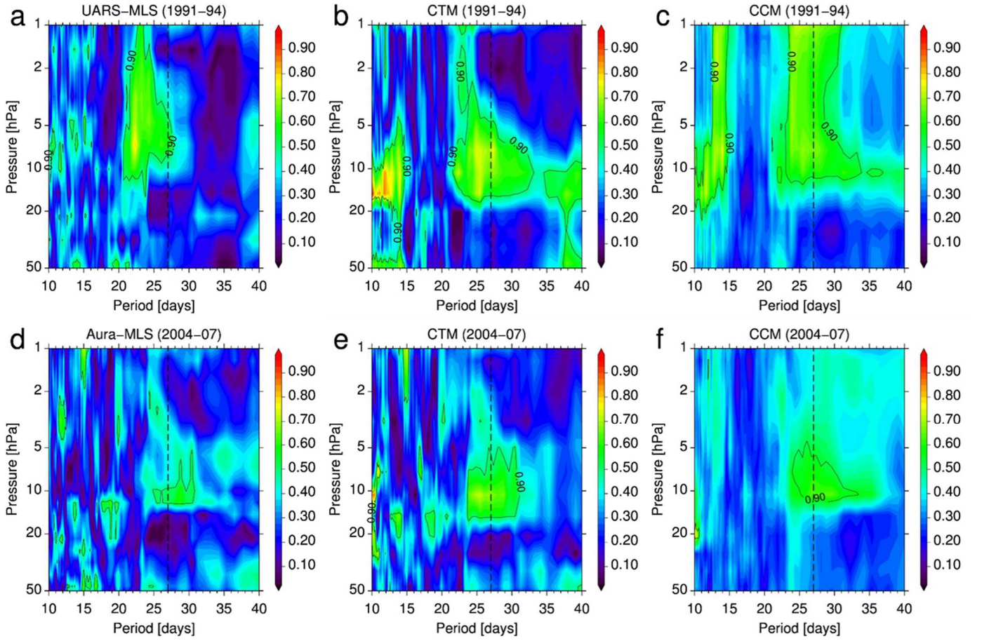
Figure 4: Mean squared coherence between ozone and F205 as a function of period (days) and pressure level (hPa) for the (top) 1991-94 and (bottom) 2004-07 period and for (a, d) MLS observations, (b,e) CTM and (c,f) CCM simulations. Black contour lines indicate the 90% confidence level and the vertical dashed black lines indicate the 27day period.
