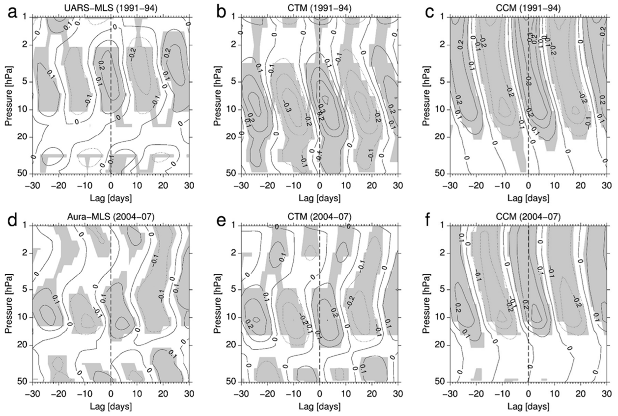
Figure 6: Cross-correlation between digitally filtered (see main text) ozone and F205 as a function of time lag (in days) and pressure level (hPa) for the (top) 1991-94 and (bottom) 2004-07 periods. (a,d), (b,e) and (c,f) panels show cross-correlation between F205 and MLS observations, CTM and CCM simulations, respectively. Shading represents areas with 95% confidence level.
