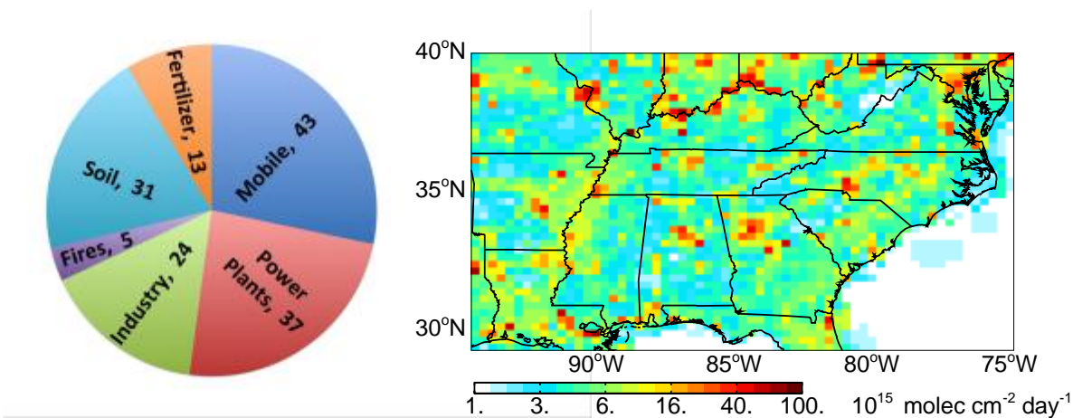
5 Figure 1: Surface \text{NO}_x emissions in the Southeast US in GEOS-Chem for August and September 2013 including fuel combustion, soils, fertilizer use, and open fires (total emissions=153 Gg N). Anthropogenic emissions from mobile sources and industry in the National Emission Inventory (NEI11v1) for 2013 have been decreased by 60% to match atmospheric observations (see text). Lightning contributes an additional 25 Gg N to the free troposphere (not included in the Figure). The emissions are mapped on the 0.25^\circ \times 0.3125^\circ GEOS-Chem grid. The pie chart gives the sum of August-September 2013 emissions (Gg N) over the Southeast US domain as shown on the map (94.5 - 75° W, 29.5-40° N).
