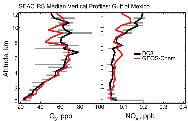
5 Figure 11: Median vertical profiles of ozone and NO x concentrations over the Gulf of Mexico during SEAC 4 RS. Observations are from four SEAC 4 RS flights over the Gulf of Mexico (August 12, September 4, 13, 16). GEOS-Chem model values are sampled along the flight tracks. The 25 th and 75 th percentiles of the aircraft observations are shown as horizontal bars.
