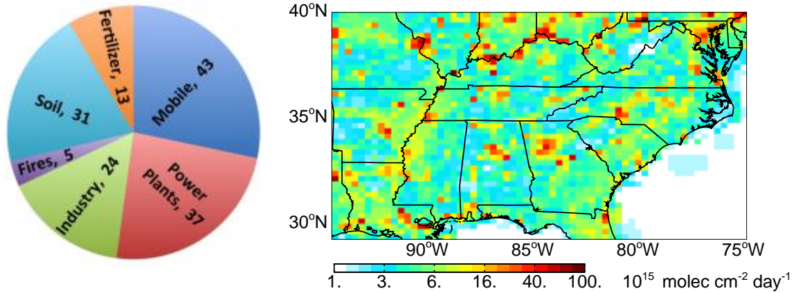
5 Figure 1: Surface NO x emissions in the Southeast US in GEOS-Chem for August and September 2013 including fuel combustion, soils, fertilizer use, and open fires (total emissions=153 Gg N). Anthropogenic emissions from mobile sources and industry in the National Emission Inventory (NEI11v1) for 2013 have been decreased by 60% to match atmospheric observations (see text). Lightning contributes an additional 25 Gg N to the free troposphere (not included in the Figure). The emissions are mapped on the 0.25° × 0.3125° GEOS-Chem grid. The pie chart gives the sum of August-September 2013 emissions (Gg N) over the Southeast US domain (94.5 - 75° W, 29.5-40° N).
