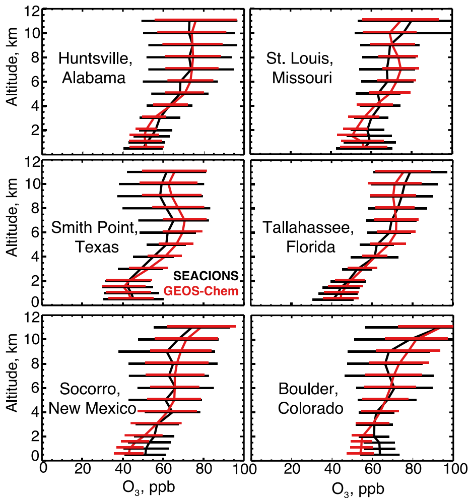
Figure 8: Mean ozonesonde vertical profiles at the USSEACIONS sites ( http://croc.gsfc.nasa.gov/seacions/ ) during the SEAC 4 RS campaign in August-September 2013. An average of 20 sondes were launched per site between 9am and 4pm local time. Ozonesondes at Smith Point, Texas were only launched in September. Model values are coincident with the launches. Data are averaged vertically over 0.5 km bins below 2 km altitude and 1.0 km bins above. Also shown are standard deviations.
