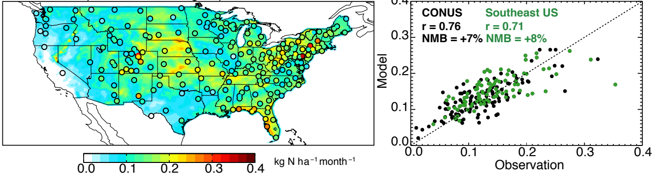
Figure 4: Nitrate wet deposition fluxes across the US in August-September 2013. Observations Mean observations from the NADP network (circles in the left panel) are compared to model values with decreased \text{NO}_x emissions (background). Also shown is a scatterplot of simulated versus observed values at individual sites for the whole contiguous US (black) and for the Southeast US (green). The correlation coefficient ( r ) and normalized mean bias (NMB) are shown inset, along with the 1:1 line.
