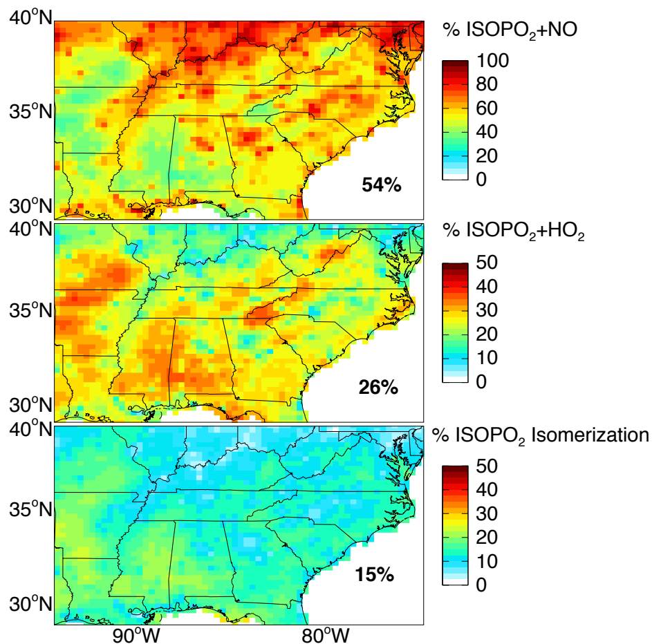
Figure 8: Branching ratios for the fate of the isoprene peroxy radical (ISOPO 2 ) as simulated by GEOS-Chem over the Southeast US for August-September 2013. Values are percentages of ISOPO 2 that react with NO, HO 2 , or isomerize from the total mass of isoprene reacting over the domain. Note the difference in scale between the top panel and the lower two panels. Regional mean percentages for the Southeast US are shown inset. They add up to less than 100% because of the small ISOPO 2 sink from reaction with other organic peroxy radicals (RO 2 ).
