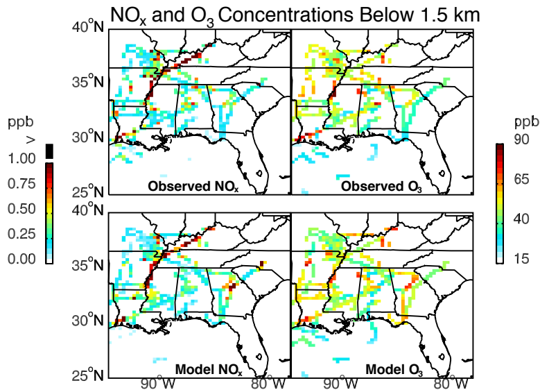
Figure 5: Ozone and \text{NO}_x concentrations in the boundary layer (0-1.5km) during SEAC 4 RS (6 Aug to 23 Sep 2013). Observations from the aircraft and simulated values are averaged over the 0.25^\circ \times 0.3125^\circ GEOS-Chem grid. \text{NO}_x above 1ppb is shown in black. The spatial correlation coefficient is 0.71 for both \text{NO}_x and \text{O}_3 . The normalized mean bias is -11.5% for \text{NO}_x and 4.5% for \text{O}_3 .
