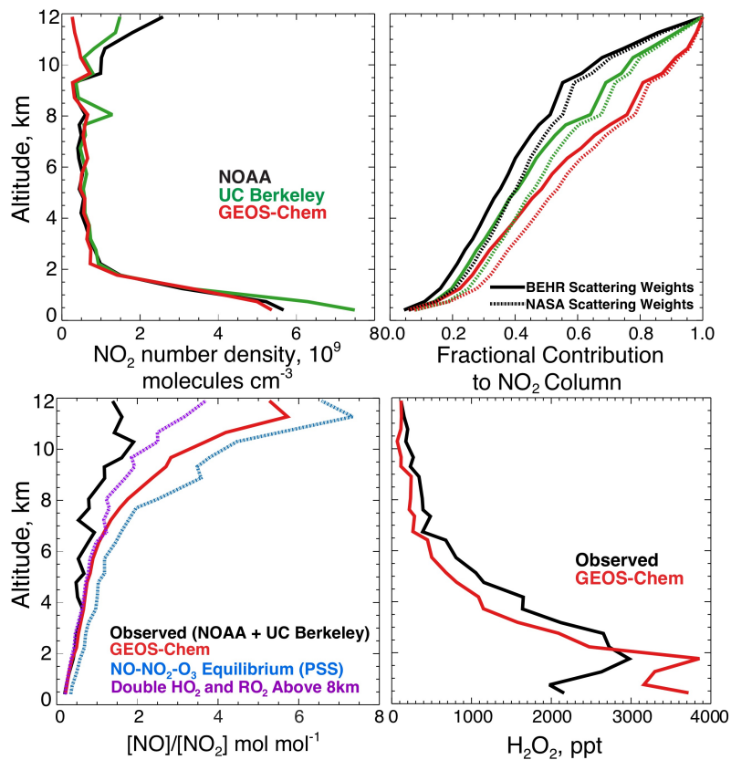
Figure 7: Vertical distribution of \text{NO}_2 over the Southeast US during SEAC 4 RS (August-September 2013) and contributions to tropospheric \text{NO}_2 columns measured from space by OMI. The top left panel shows median vertical profiles of \text{NO}_2 number density measured from the SEAC 4 RS aircraft by the NOAA and UC Berkeley instruments and simulated by GEOS-Chem. The middle top right panel shows the fractional contribution of \text{NO}_2 below a given altitude to the total tropospheric \text{NO}_2 slant column measured by OMI, accounting for increasing sensitivity with altitude as determined from the retrieval scattering weights. The right bottom left panel shows the mean median vertical profiles of the daytime [\text{NO}]/[\text{NO}_2] molar concentration ratio in the aircraft observations (NOAA for NO and UC Berkeley for \text{NO}_2 ) and in GEOS-Chem. Also shown is the ratio computed from NO- \text{NO}_2 - \text{O}_3 photochemical steady state (PSS) as given by reactions (5)+(7) (blue) and including reaction (6) with doubled \text{HO}_2 and \text{RO}_2 concentrations above 8km (purple). The bottom right panel shows the median \text{H}_2\text{O}_2 profile from the model and from the SEAC 4 RS flights over the Southeast US. \text{H}_2\text{O}_2 was measured by the Caltech CIMS (see Figure 2).
