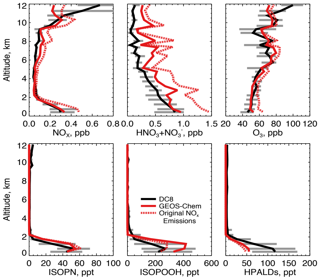
Figure 3: Median vertical concentration profiles of \text{NO}_x , total inorganic nitrate (gas \text{HNO}_3 + aerosol \text{NO}_3^- ), ozone, isoprene nitrate (ISOPN), isoprene hydroperoxide (ISOPOOH), and hydroperoxyaldehydes (HPALDs) for the SEAC 4 RS flights over the Southeast US (domain of Figure 1). Observations from the DC-8 aircraft are compared to GEOS-Chem model results. The dashed red line shows model results before sealing adjustment of \text{NO}_x emissions from fuel combustion and lightning- (see text). The 25 th and 75 th percentiles of the DC-8 observations are shown as grey bars. The SEAC 4 RS observations have been filtered to remove open fire plumes, stratospheric air, and urban plumes as described in the text. Model results are sampled along the flight tracks at the time of flights and gridded to the model resolution. Profiles are binned to the nearest 0.5 km. The NOAA \text{NO}_y\text{O}_3 4-channel chemiluminescence (CL) instrument made measurements of ozone and \text{NO}_y (Ryerson et al., 1998), NO (Ryerson et al., 2000) and \text{NO}_2 (Pollack et al., 2010). Total inorganic nitrate was measured by the University of New Hampshire Soluble Acidic Gases and Aerosol (UNH SAGA) instrument (Dibb et al., 2003) and was mainly gas-phase \text{HNO}_3 for the SEAC 4 RS conditions. ISOPOOH, ISOPN, and HPALDs were measured by the Caltech single mass analyzer CIMS (Crouse et al., 2006; Paulot et al., 2009a; Crouse et al., 2011).
