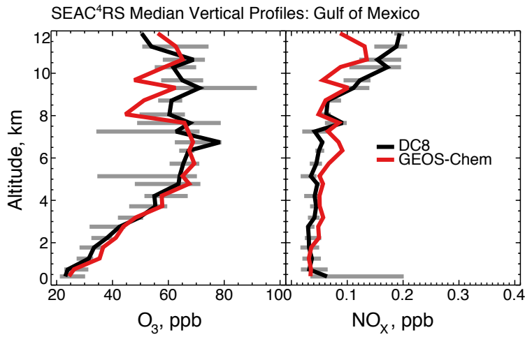
Figure 12: Median vertical profiles of ozone and NO x concentrations over the Gulf of Mexico during SEAC 4 RS. Observations are from four SEAC 4 RS flights over the Gulf of Mexico (August 12, September 4, 13, 16). GEOS-Chem model values are sampled along the flight tracks. The 25 th and 75 th percentiles of the aircraft observations are shown as horizontal bars.
