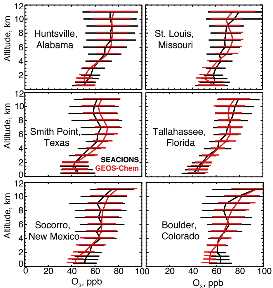
Figure 9: Mean ozonesonde vertical profiles at the US SEACIONS sites ( http://croc.gsfc.nasa.gov/seacions/ ) during the SEAC 4 RS campaign in August-September 2013. An average of 2520 2520 sondes were launched per site between 11am 9am and 2pm 4pm local time. Ozonesondes at Smith Point, Texas were only launched in September. Model values are coincident with the launches. Data are averaged vertically over 0.5 km bins below 2 km altitude and 1.0 km bins above. Also shown are standard deviations.
