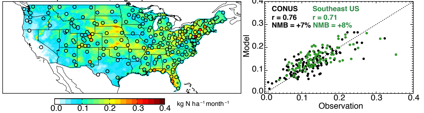
Figure 3: Nitrate wet deposition fluxes across the US in August-September 2013. Observations Mean observations from the NADP network (circles in the left panel) are compared to model values with decreased \text{NO}_x emissions (background). Also shown is a scatterplot of simulated versus observed values at individual sites for the whole contiguous US (black) and for the Southeast US (green). The correlation coefficient ( r ) and normalized mean bias (NMB) are shown inset, along with the 1:1 line.
