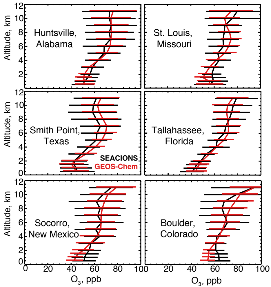
Figure 8: Mean ozonesonde vertical profiles at the US SEACIONS sites ( http://croc.gsfc.nasa.gov/seacions/ ) during the SEAC 4 RS campaign in August-September 2013. An average of 2520 sondes were launched per site between 11am-9am and 2pm-4pm local time. Ozonesondes at Smith Point, Texas were only launched in September. Model values are coincident with the launches. Data are averaged vertically over 0.5 km bins below 2 km altitude and 1.0 km bins above. Also shown are standard deviations.
