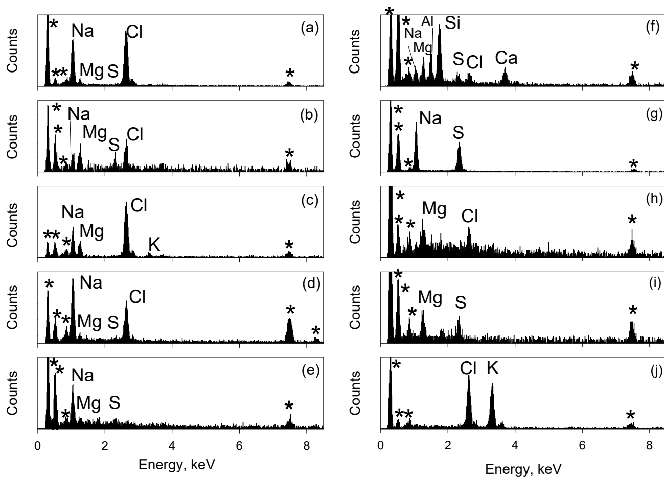
Figure 8 EDX spectra of sea-salt particles and sea-salt relating particles collected over the sea-ice area. Asterisks denote background peaks derived from the sample substrate.
