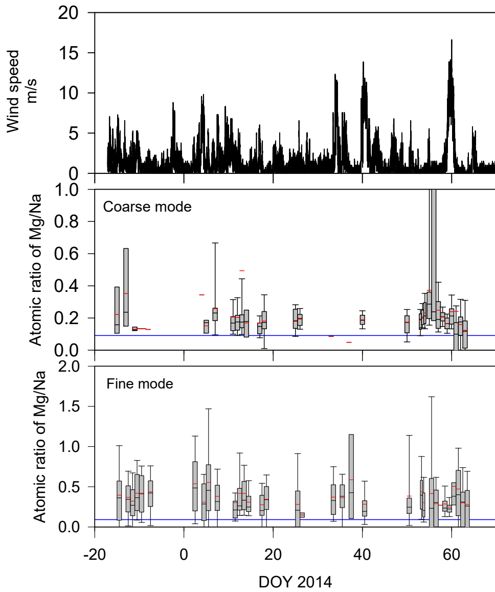
Figure 11 Variations of wind speed and atomic ratios of Mg/Na in sea-salt particles and the modified sea-salt particles collected over the sea-ice area. In box plots, the top bar, top box line, black middle box line, bottom box line, and bottom bar respectively denote values of 90, 75, 50 (median), 25, and 10%. The red and lines show mean values and seawater ratio of Mg/Na.
