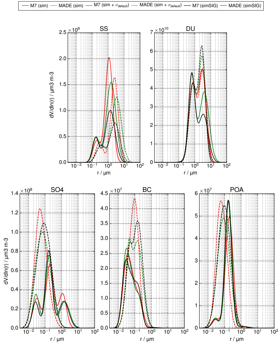
Figure 5. Domain-averaged volume distributions for different species and standard deviations. Distributions are obtained by weighting the total dry volume distribution by the fraction the respective species contributes to the total mass. The total distribution is the sum of all model modes, which are determined from the vertical sum and horizontal averages of the corresponding dry masses and numbers. Species include sea salt (SS), dust (DU), sulfate ( \text{SO}_4 ), soot (BC) and primary organic carbon (POA). Individual lognormal modes are determined from the vertical sum and horizontal average of the corresponding dry masses and numbers. The full, multimodal distribution emerges as the sum of individual log-normal modes. For mixed modes, lognormal modes of individual species are obtained by weighting the mixed-modal distribution by the fraction that the respective species contributes to the total mass in the mixed mode. The figure compares simulations sim , generated with the universal standard deviation \sigma_{\text{universal}} = 1.7 for all modes (red), simulations sim but plotted using default standard deviations \sigma_{\text{default}} as given in Table 1 (green) and simulations simSIG , generated with \sigma_{\text{default}} (black).
