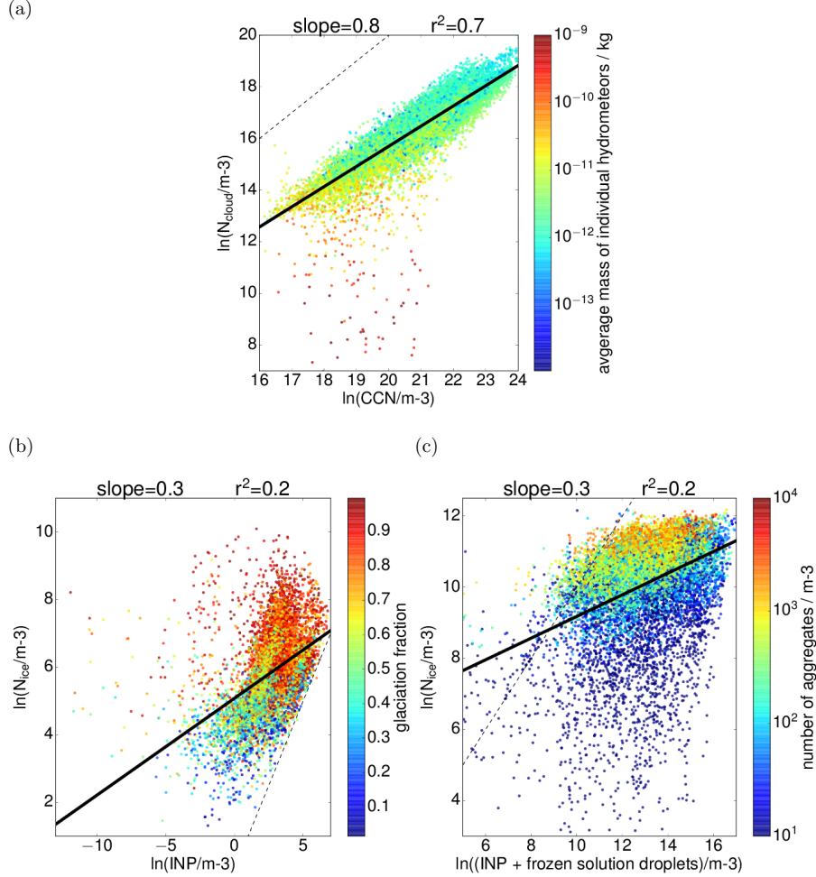
Figure 14. Relationship between CCN/INP and cloud droplet number concentration N_{\text{cl}} and ice crystal number concentration N_{\text{ci}} . The figures show double logarithmic scatter plots of the cloud droplet number concentration N_{\text{cl}} as function of CCN concentration in liquid clouds (a) and the ice crystal number concentration N_{\text{ci}} as function of INP concentration in mixed-phase clouds (b) and as function of the combined concentration of INP + frozen solution droplets in cirrus clouds (c). Warm and mixed-phase clouds are defined as in Figures 10 and 12, cirrus clouds are restricted to regions with competition of heterogeneous and homogeneous freezing as indicated by non-vanishing numbers of both, INP and solution droplets. Data points represent temporally and vertically averaged values from coupled simulations with the Phillips ice nucleation parameterization at every grid point (see text for details). Only every 5th data point used for the fit is displayed. Solid black lines illustrate least-square fits with slope and coefficient of determination r^2 as indicated in plot titles. All fits are significant. Black dashes indicate one-to-one lines. Colors denote the mass of individual hydrometeors, averaged over all cloud droplets and rain drops (a), the glaciation fraction, i. e. the ratio of frozen to total cloud water (b), and the number of ice-crystal aggregates (c).
