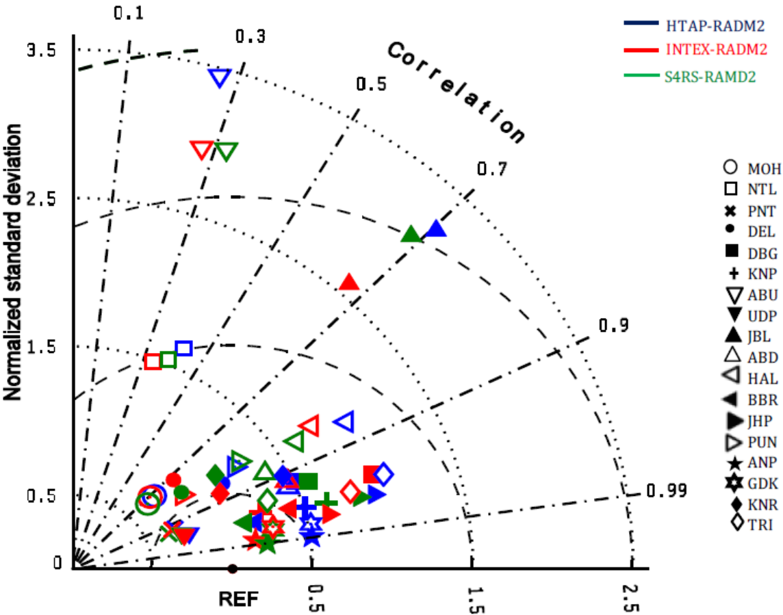
976 Figure 7. Taylor diagram with summary model statistics ( r , normalized standard deviation and RMSD) at all sites. The 977 correlation is the cosine of the angle from the horizontal axis, the root mean square difference is the distance from the reference 978 point (REF) and the standard deviation is the distance from the origin.
