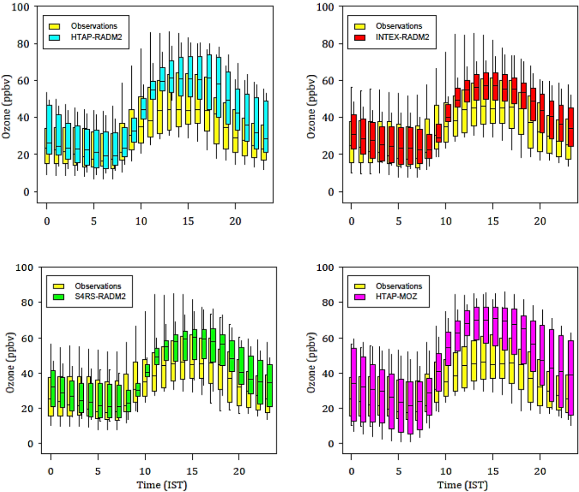
1051 Figure 13. Box/whisker plot comparison of monthly average diurnal variation of surface ozone from model runs and 1052 observations over the entire domain (after spatially averaging the results). Upper and lower boundaries of boxes denote the 1053 75th and 25th percentiles and whiskers represent the 95th and 5th percentiles. The line in the box is the median.
