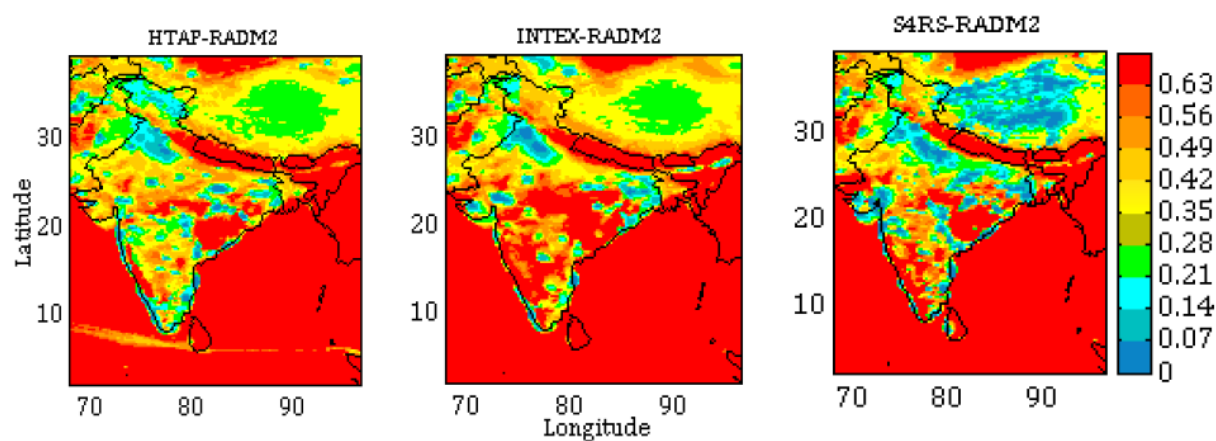
Figure 5. Net daytime surface \text{CH}_2\text{O} to \text{NO}_y ratio in simulations with different inventories for the month April during 0630-1230 IST.
