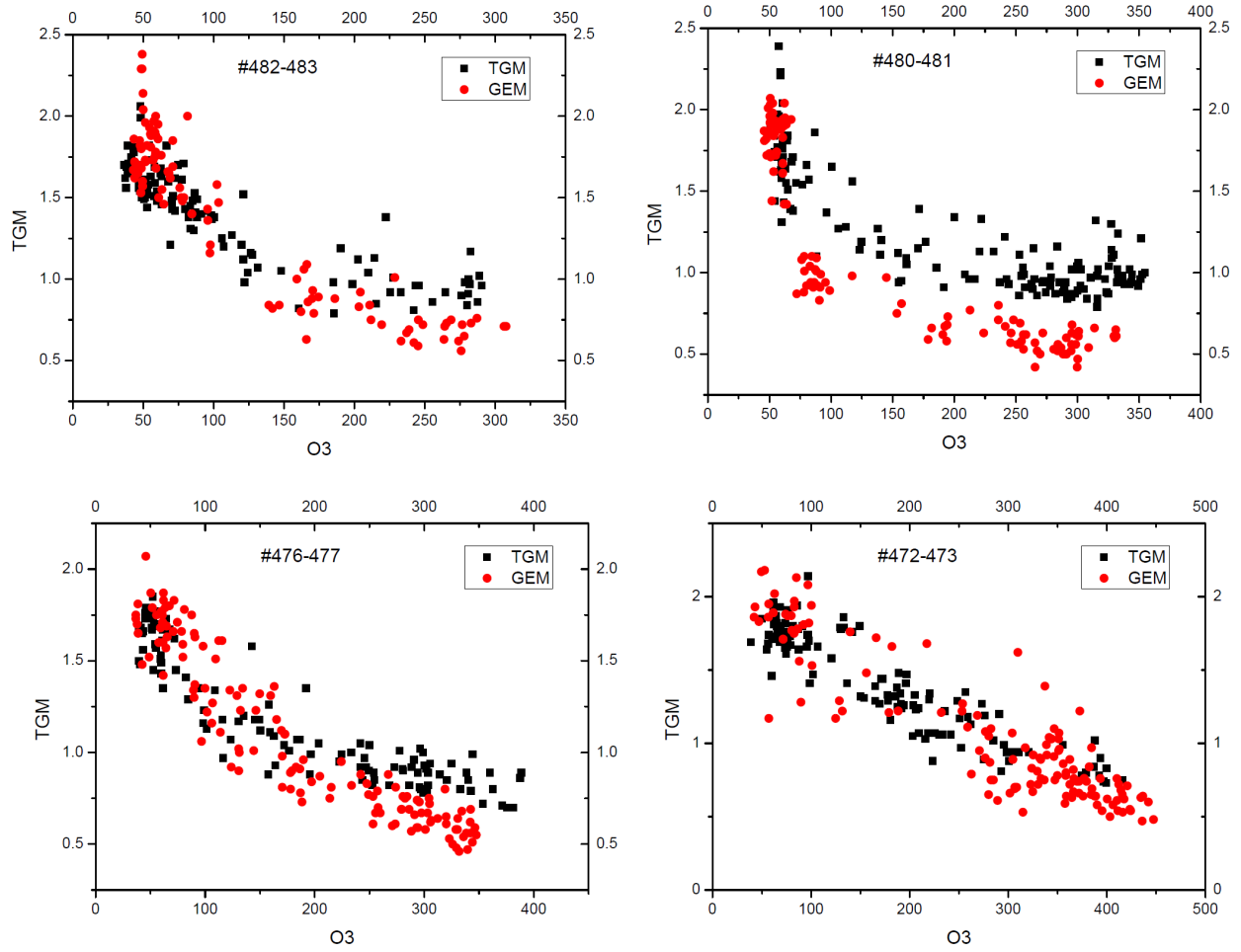
Figure S1: Scatter plot of GEM and TGM measurements from intercontinental CARIBIC flights. On the outward flight TGM and on the return flight GEM was measured.
