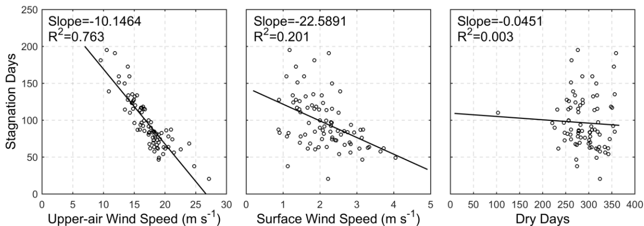
Figure 8. Dependence of spatial distribution of stagnation days on three components (upper-air wind speed, surface wind speed and dry days). Linear regression coefficients between annual mean stagnation days at 81 stations and each corresponding component are shown.
