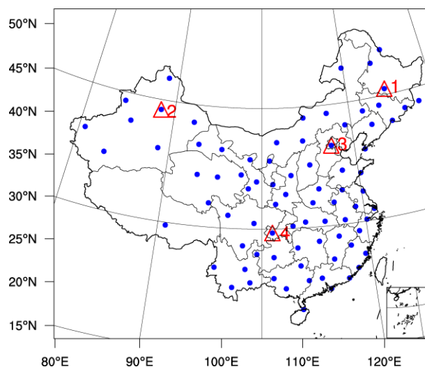
5 Figure 1. Distribution of observation stations. Triangles indicate four stations selected to discuss seasonal variations of air stagnations in Section 3: 1 for Harbin, 2 for Urumqi, 3 for Beijing, 4 for Chongqing.
