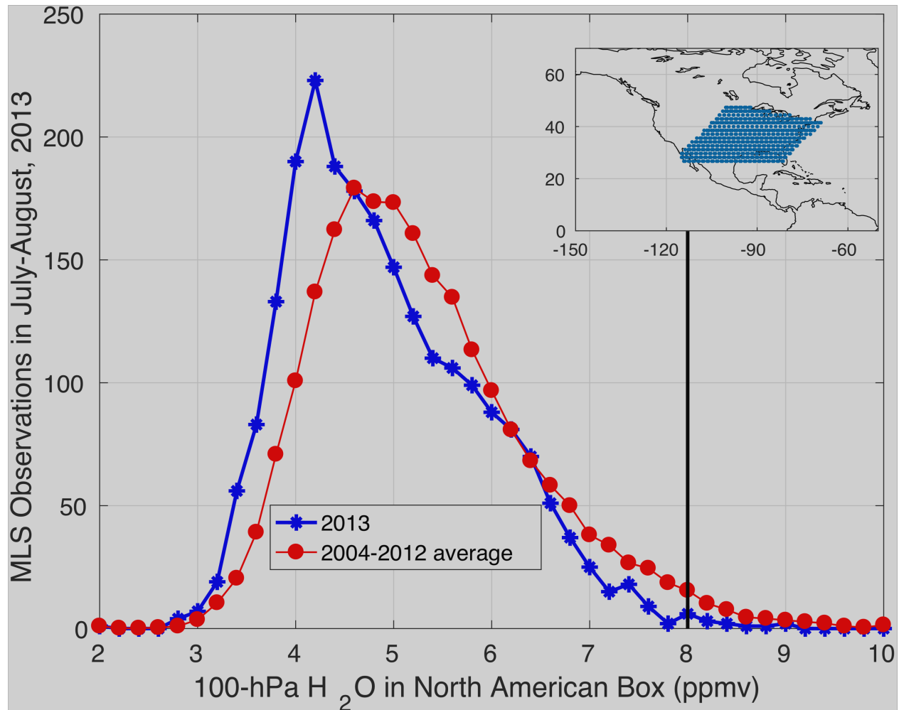
Figure 4. Distribution of Aura MLS v4.2 100-hPa H 2 O over CONUS (blue shaded box in insert), corresponding to approximately 17 km altitude. The two histograms for July-August 2013 (blue asterisks and trace) and the previous nine-summer MLS record, July-August 2004 through 2012 (red circles and trace) indicates that 2013 was drier than average. The threshold for MLS-detected ‘enhanced water vapor’ (thick black vertical line) is set at 8 ppmv, same as Schwartz et al. (2013), to exclude the larger population of measurements at 6 to 8 ppmv water vapor that may have other sources.
