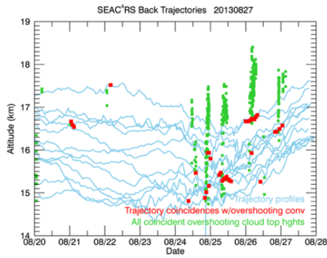
Figure 9. Analysis of the 27 August 2013 NASA ER-2 flight. (a) Vertical profiles of JLH Mark2 in situ H 2 O similar to Figure 7a, (b) Back trajectories from the aircraft path similar to Figure 7b, (c) Altitude plot of back trajectories showing coincident overshooting (red) and and all overshooting within +/- 3 hours (green) similar to Figure 7c, (d) Days between OT and intercept by aircraft similar to Figure 7d.
