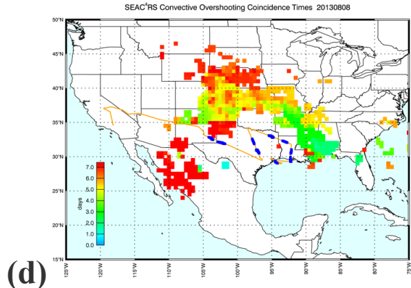
Figure 7. Analysis of the 8 August 2013 NASA ER-2 aircraft flight. (a) Vertical profiles of JLH Mark2 in situ H 2 O. Back trajectories were initialized from all aircraft water measurements at 16 to 17.5 km altitude. (b) Example back trajectories (thin blue traces) and coincident overshooting convection (red). Along the NASA ER-2 flight track (orange line), enhanced water vapor was measured (thick blue lines). This figure identifies where trajectories and OT are coincident (red squares) within tolerances prescribed in Section 3.2. The green markers are overshooting convective tops within +/-3 hours of the red squares to indicate the main regions of convective overshooting during the seven days prior to the ER-2 flight and which of those regions appeared to contribute most to the water vapor enhancement measured on the flight. (c) Altitude plot of example back trajectories showing coincident overshooting (red squares). The green markers are overshooting convective tops within +/-3 hours of the red squares. The high resolution of the convective overshooting data meant that there could be multiple coincident convective overshooting cells for a single location on a back trajectory, (d) Days between OT and intercept by aircraft on 8 August 2013.
