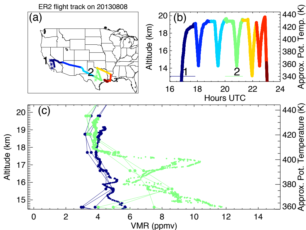
Figure 6. Map and profiles of aircraft and satellite water vapor on 8 August 2013 over California (number 1 shown in dark blue) and Texas (number 2 shown in green). (a) Map of ER-2 aircraft flight track (solid colored trace) and nearly coincident Aura MLS geolocations (asterisks and lines). (b) ER-2 aircraft altitude profiles (solid colored trace) color-coded by dives and MLS times (horizontal lines). (c) Vertical profiles of in situ water vapor measurements from JLH Mark2 (dots) and MLS retrievals of water vapor (circles and lines). Some measurements exceed the threshold for enhanced water vapor of 8 ppmv for Aura MLS (after Schwartz et al., 2013), and the campaign-wide mean plus 2 st. dev. for JLH Mark 2, 9.7 ppmv at 380–400 K and 6.6 ppmv at 400–420 K.
