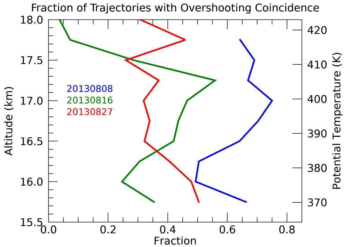
Figure 10. Fraction of back trajectories that intersected OTs during the 7 previous days for the three SEAC 4 RS flights of 8 August (blue), 16 August (green) and 27 August 2013 (red) shown in Figures 7, 8 and 9, respectively.
