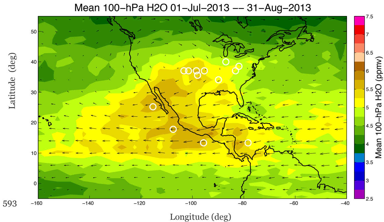
Figure 5. Two-month mean map of Aura MLS v4.2 100-hPa H 2 O (color scale), corresponding to approximately 17 km altitude, with superimposed MERRA horizontal winds (arrows) for July-August 2013 during the SEAC 4 RS time period. MLS observations of 100-hPa H 2 O greater than 8 ppmv in this two-month period are shown by the white circles.
