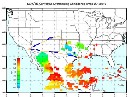
Figure 8. Analysis of the 16 August 2013 NASA ER-2 flight. (a) Vertical profiles of JLH Mark2 in situ H 2 O similar to Figure 7a, (b) Back trajectories from the aircraft path similar to Figure 7b, (c) Altitude plot of back trajectories showing coincident overshooting (red) and all overshooting within +/- 3 hours (green) similar to Figure 7c, (d) Days between OT and intercept by aircraft similar to Figure 7d.
