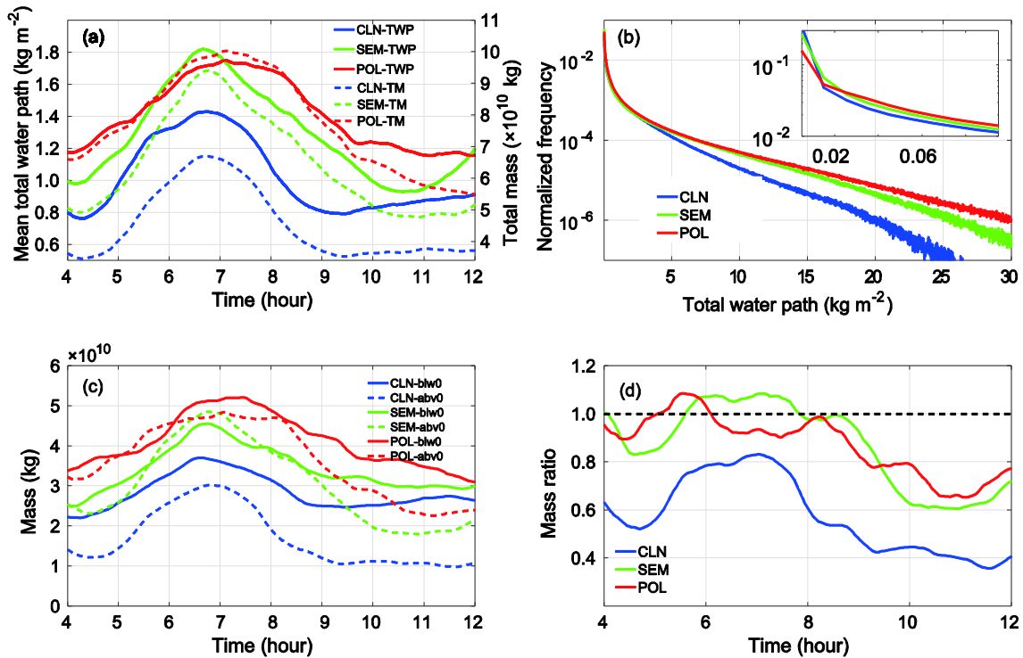
210 Fig. 4 (a) Time series of the mean total water path (TWP, \text{kg m}^{-2} ) over the cloudy area (solid curves) and the total cloud mass (kg, dashed curves). (b) Normalized occurrence-frequency distribution of TWP over the domain during 4 to 12 h of the simulation. Time series of (c) total cloud mass above (dashed curves) and below (solid curves) the ZTL and (d) the mass ratios for clean (blue curves), semi-polluted (green curves), and polluted (red curves) simulations.
