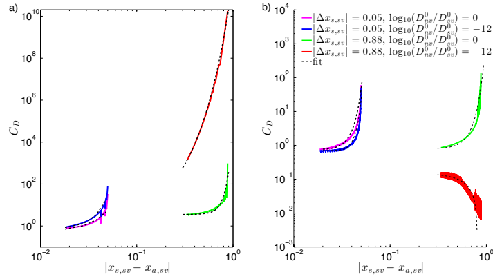
Figure 3. Examples of the correction factor for D in the analytical solution ( C_D ) required to give agreement with radius estimates in Fi-PaD as a function of proximity to equilibrium. a) and b) are for +ve \Delta x_{s,sv} and -ve \Delta x_{s,sv} , respectively. The model scenario is described in the legend, which applies to both plots. Fits are plotted using eq. 9.
