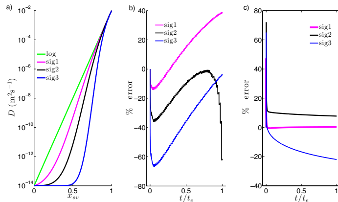
Figure 11. Plot a) shows the logarithmic dependency of diffusion coefficient on mole fraction on which the presented correction is derived and the sigmoidal dependencies for which it was tested. In b) and c) are the analytical model errors (eq. 10) when the sigmoidal dependencies given in a) were used. b) +ve \Delta x_{s,sv} and c) -ve \Delta x_{s,sv} , and for both plots |\Delta x_{s,sv}| = 0.88 and \log_{10}(D_{nv}^0/D_{sv}^0) = -12 .
