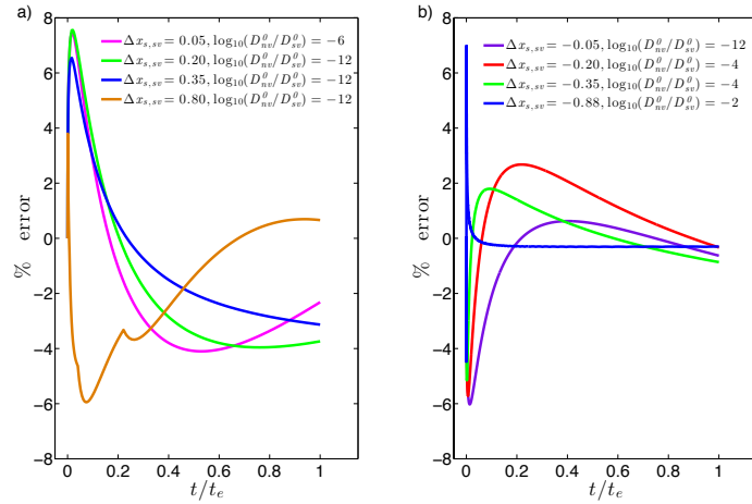
Figure 4. Examples of % error (eq. 10) of the analytical model with corrected D when diffusion is composition-dependent (eq. 2), plotted against time normalised by the e -folding time. a) and b) are for +ve \Delta x_{s,sv} and -ve \Delta x_{s,sv} , respectively, and scenarios are given in the legend.
