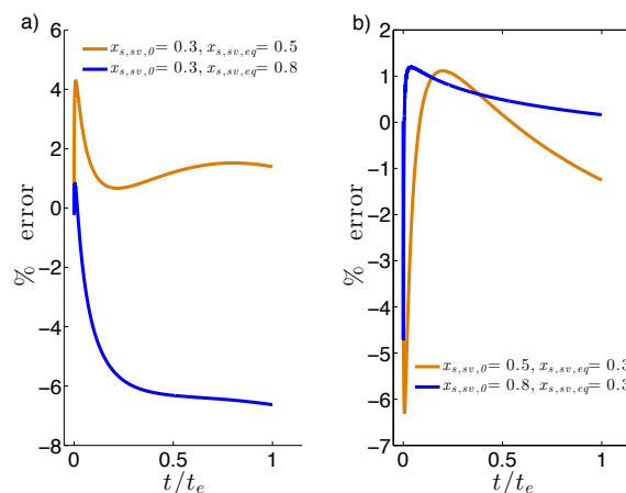
Figure 7. Agreement between corrected analytical and Fi-PaD estimates, using the metric given in eq. 10, for: a) +ve \Delta x_{s,v} and b) -ve \Delta x_{s,v} , as shown in the legend. The start/finish x_{s,v} \neq 0 for a)/b), therefore the transformation to an effective model setup (as described in the main text) was required. For both a) and b) \log_{10}(D_{nv}^0 / D_{sv}^0) = -12 .
