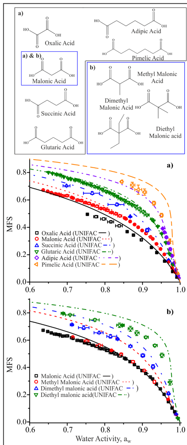
Fig. 2. Equilibrium hygroscopic growth curves are shown in (a) for the homologous series of straight chain dicarboxylic acids and in (b) for dicarboxylic acids with a malonic acid backbone and increasing methyl substitution.
