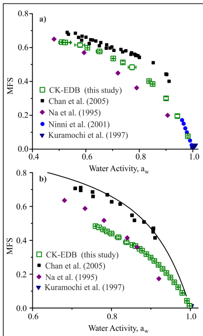
Figure 9. Equilibrium hygroscopicity data for (a) glycine and (b) alanine. The UNIFAC model prediction for alanine is also shown (solid black line).
