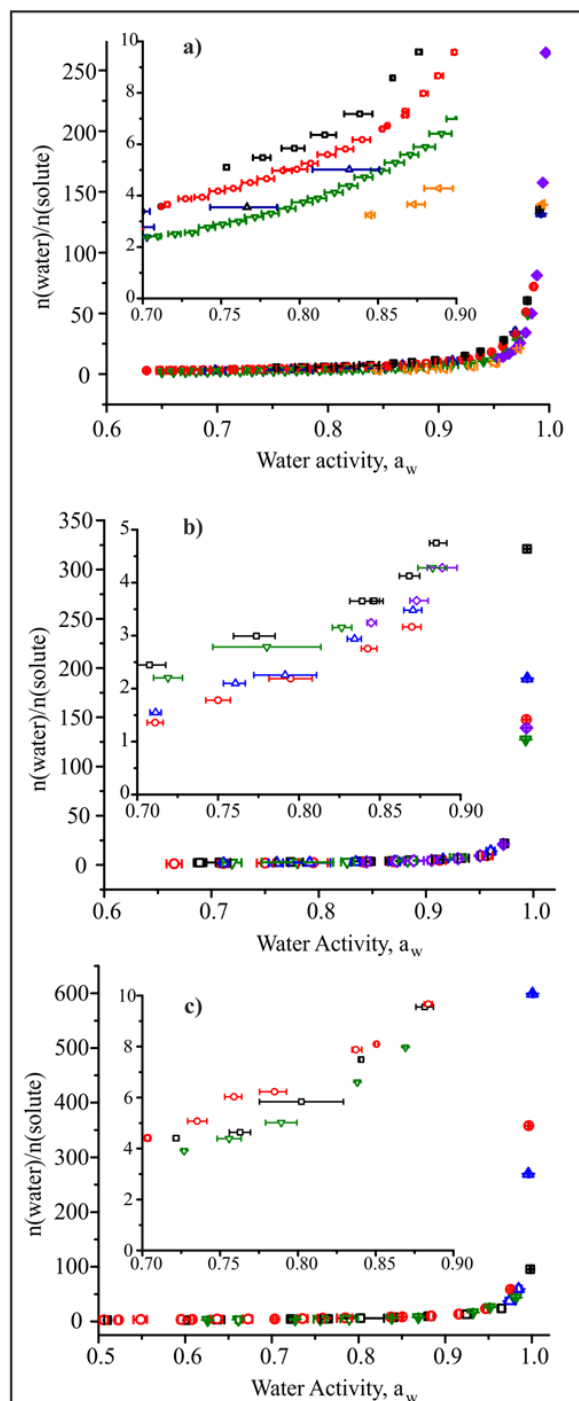
Figure 6. Moles of water, per mole of solute for (a) for straight chain dicarboxylic acids for oxalic (black squares), malonic acid (red circles), succinic acid (blue up triangles), glutaric acid (green down triangles), adipic acid (violet diamonds) and pimelic acid (orange left triangles). In (b) for diethylmalonic acid (black squares), 2,2-dimethyl glutaric acid (red circles), 3,3-dimethyl glutaric acid (blue triangles), 3-methyl adipic acid (pink down triangles) and pimelic acid (green diamonds). And in (c) for galactose (black squares), sorbitol (red circles), xylose (blue down triangles) and erythritol (green down triangles).
