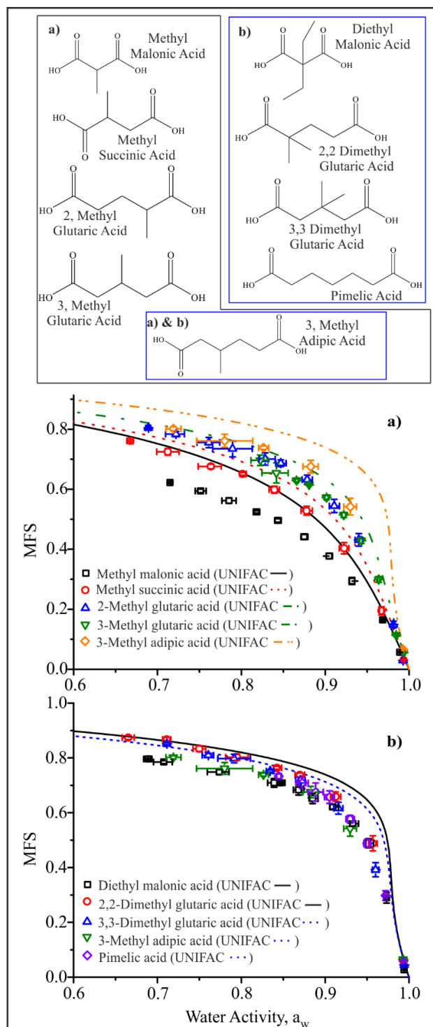
Figure 5. Equilibrium hygroscopicity curves for a series of branched dicarboxylic acids are shown in a). In (b) CK-EDB hygroscopicity curves for a series of dicarboxylic acids with the same O:C ratio of 0.57.
