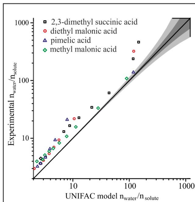
Figure 7. Comparison of the experimentally determined number of moles of water per mole of solute and the value predicted from UNIFAC for the four dicarboxylic acids with the largest deviation from UNIFAC. Shaded regions correspond to error in a_w of \pm 0.001 (dark shaded grey regions) and \pm 0.002 (light shaded grey regions).
