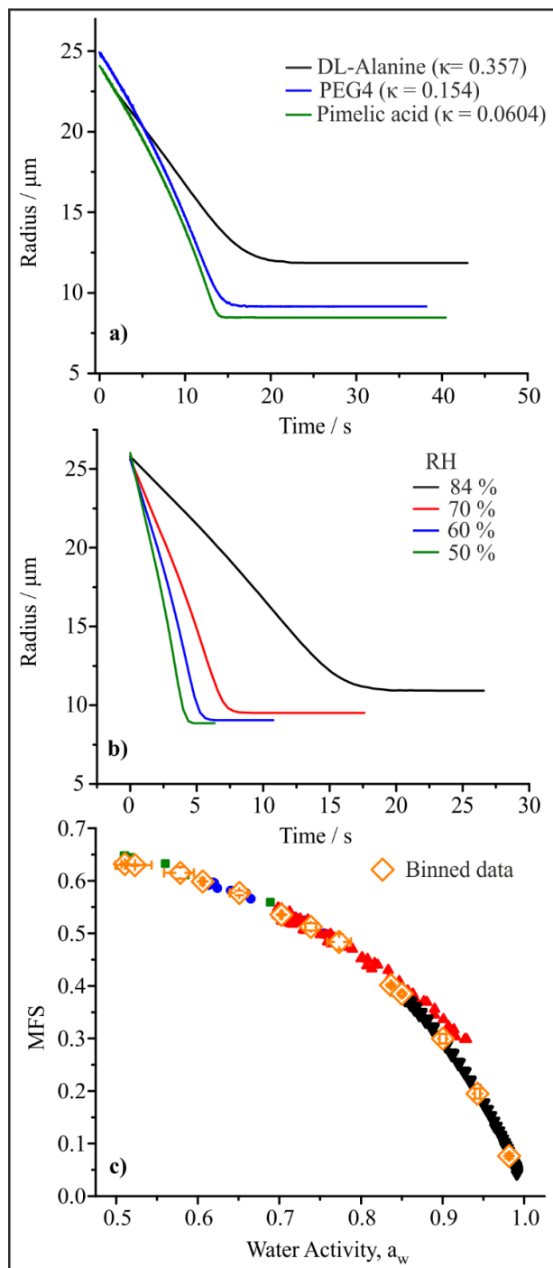
Fig. 1. (a) Examples of the time-dependent evaporation of aqueous droplets containing compounds with varying \kappa value evaporating into similar RHs (~82 %). (b) The time-dependence of the radii of droplets of aqueous glycine evaporating into different RHs. (c) Equilibrium hygroscopicity curve for glycine, with binned data points (large open orange diamonds) estimate across the four different experiments at four RHs shown in (b).
