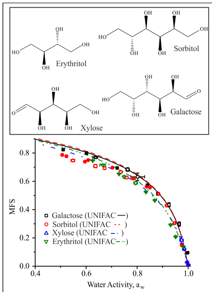
Figure 10. Equilibrium hygroscopicity curves for sugars and alcohols with the same O:C ratio of 1.
