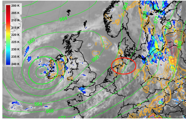
Figure 4. EUMetrain infra-red satellite image of Europe on 3 August 2012 at 12:00 UTC. Colors are cloud top temperatures showing high clouds. Green contours contour lines are geopotential height at 500 hPa and orange contour lines are CAPE-values provided from ECMWF NWP ( www.eumetrain.org ). The area of interest is marked with a red circle. Note the CAPE values within the marked area and the high clouds, which correspond to the intense precipitation.
