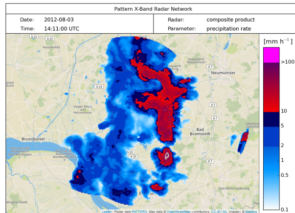
Figure 5. Radar composite from high resolution radars (Lengfeld et al., 2014) showing the precipitation rate over Htzehoe-Northern Germany on 3 August 2012 at 14:11 UTC.
