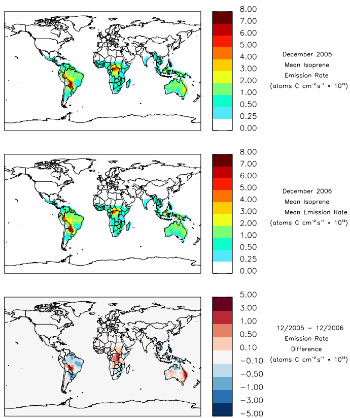
Figure 3. Monthly mean MEGAN biogenic isoprene emission rate for December 2005 (top) and December 2006 (middle). The bottom panel presents the difference in average emission rates between December 2005 and December 2006.
