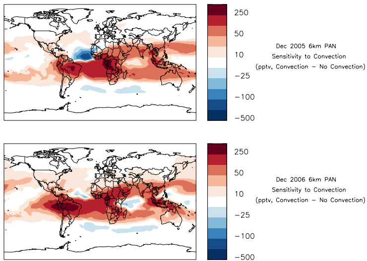
Figure 4. Sensitivity of PAN to convection during December 2005 (top) and December 2006 (bottom) at 6 km calculated as the difference in PAN between a simulation with and without convection.
