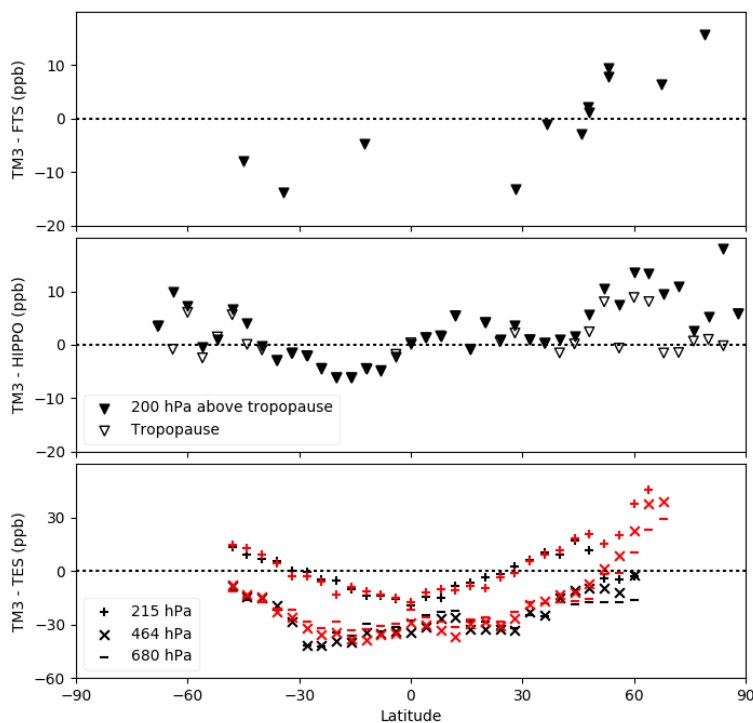
Figure 6. Comparisons of \text{CH}_4 between TM3 and (upper panel) FTS, (middle panel) HIPPO and (lower panel) TES. In the case of HIPPO and FTS the tropospheric column-averaged \text{CH}_4 is compared, which is obtained from integration between surface and the tropopause (empty characters) or 200 hPa above the tropopause shifted (solid characters, only in the HIPPO case). For TES \text{CH}_4 mole fractions at 215 hPa, 464 hPa and 680 hPa are compared with TM3 simulations in a region 110^\circ\text{W}\sim 150^\circ\text{E} (black) and the region beyond it (red) separately. Both TM3 and measurements are averaged during HIPPO 1-5 period.
