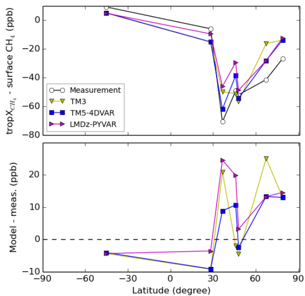
Figure 4. Measured (black) and simulated (yellow: TM3, blue: TM5-4DVAR, LMDz-PYVAR: 555 magenta) vertical gradients of CH 4 in the troposphere (top panel) and differences between the measurement and simulations (lower panel) against latitude. The results are averaged for 2007-2011 when FTS measurements are available.
