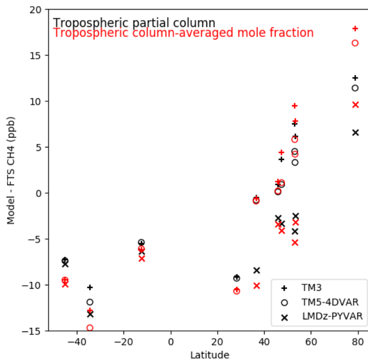
Figure A1. Latitudinal dependences of yearly averaged model biases in the tropospheric partial column (black) and the tropospheric column-averaged mole fraction (red). The three models are represented by Plus (TM3), Circle (TM5-4DVAR) and Multiplication (LMDz-PYVAR) respectively.
