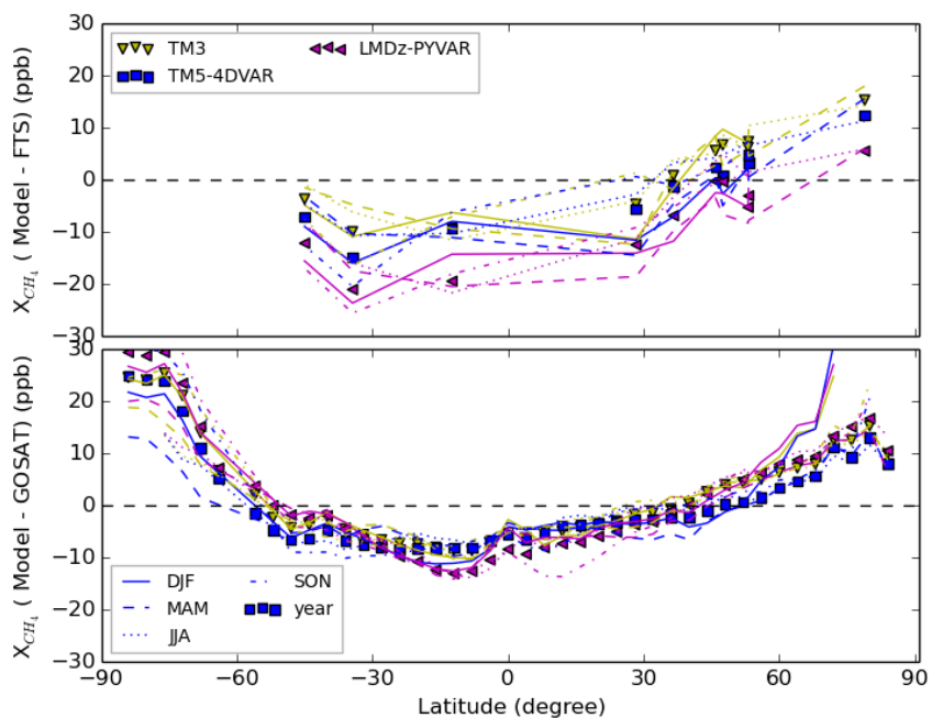
530 Figure 2. Yearly and seasonal mean model bias of total column-averaged \text{CH}_4 mole fractions plotted as a function of latitude. The upper panel is the results using FTS data while the lower panels is for GOSAT. The difference for the models is given in yellow (TM3), blue (TM5-4DVAR), and magenta (LMDz-PYVAR). The average of FTS results is for the period 2007-2011 where FTS measurements are available, and for GOSAT in the period 2009-2011.
