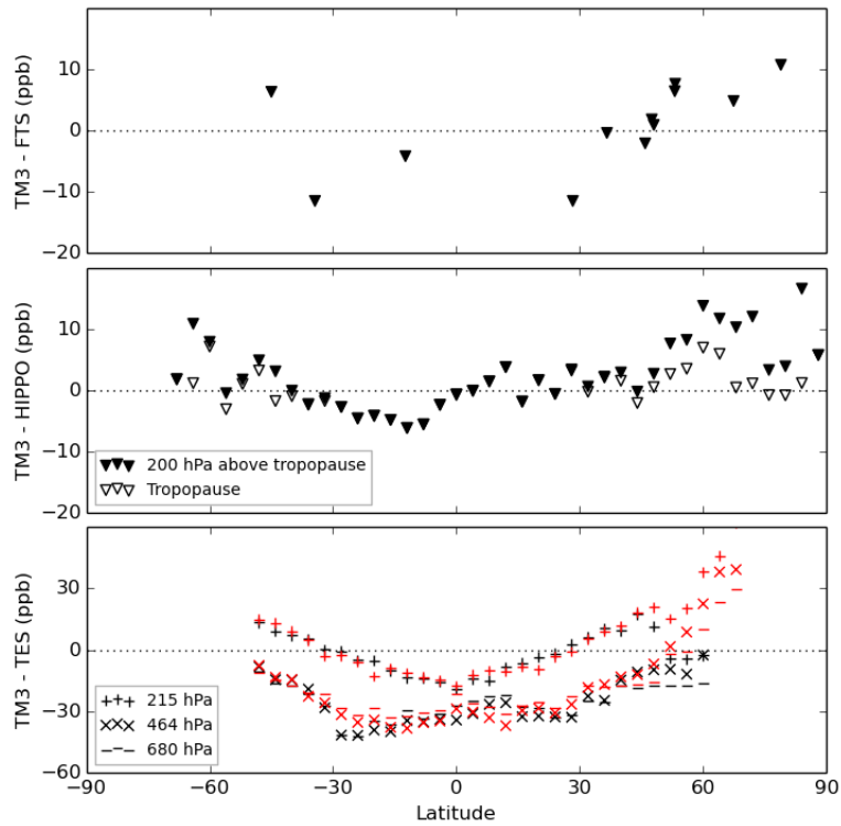
Figure 6. Comparisons of CH 4 between TM3 and (upper panel) FTS, (middle panel) HIPPO and (lower panel) TES. In the case of HIPPO and FTS tropospheric column-averaged CH 4 is compared, which is obtained from integration between surface and the tropopause (empty characters) or 200 hPa above the tropopause shifted (solid characters). For TES CH 4 mole fractions at 215 hPa, 464 hPa and 680 hPa are compared with TM3 simulations in a region 110°W~150°E (black) and the region beyond it (red) separately. Both TM3 and measurements are averaged during HIPPO 1-5 period.
