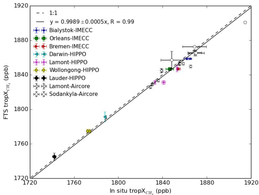
5 Figure 1. Calibration results of FTS derived tropospheric column-averaged \text{CH}_4 mole fractions against in situ measurements. The in situ profiles are smoothed using GFIT \text{CH}_4 averaging kernels in the troposphere as described in Wang et al. (2014). The FTS data are averaged for the in situ measurement periods. The IMECC is an aircraft campaign over Europe (Geibel et al., 2012). The Lamont-AirCore measurements are from Greenhouse Gas Group Aircraft Program ( http://www.esrl.noaa.gov/gmd/ccgg/aircraft/ ). The AirCore data at Sodankylä is from the FTS group 10 there.
