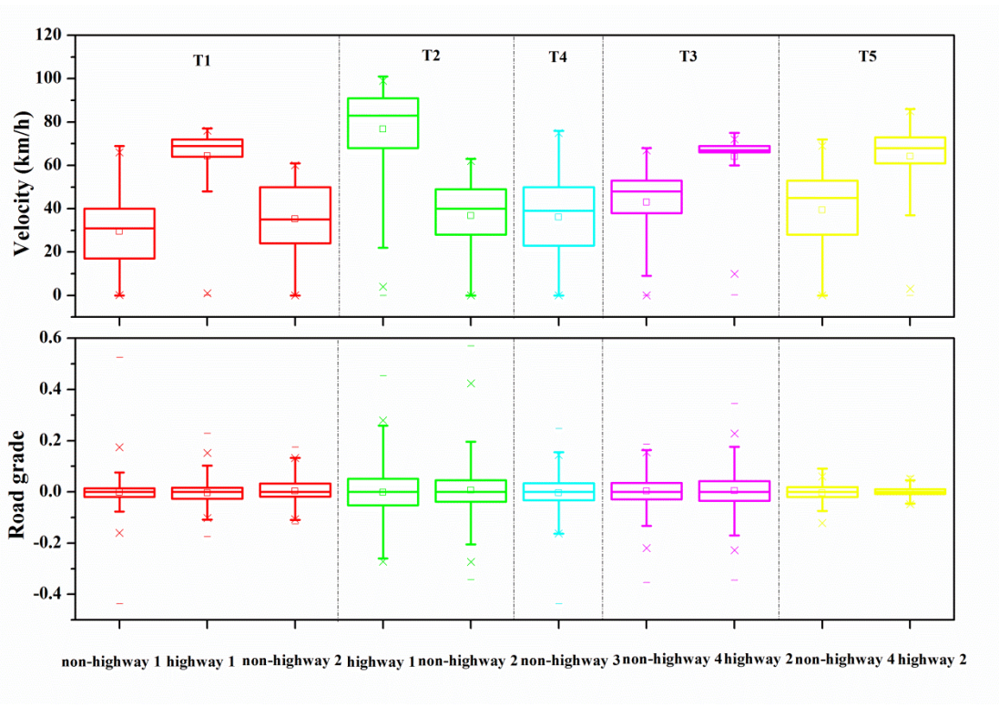
Figure S3 Box plots of velocity and road grade for different trucks under different roads
