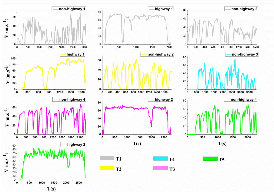
Figure S2 Velocity profiles of diesel trucks under different roads
